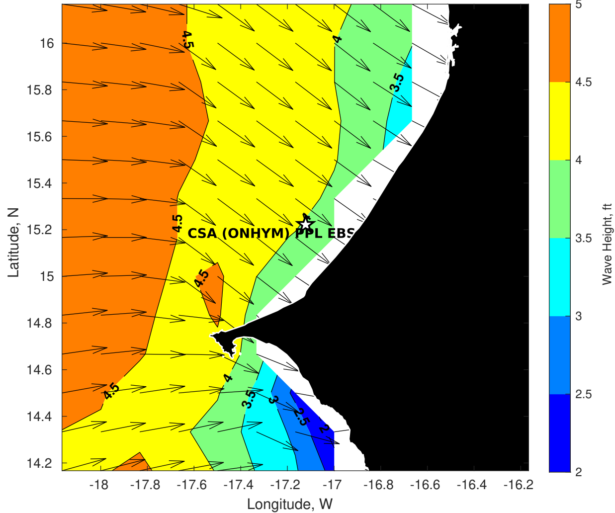
GFS Wave Height (ft) for CSA (ONHYM) PPL EBS - Senegal at 23-Nov-2025 09:00:00
