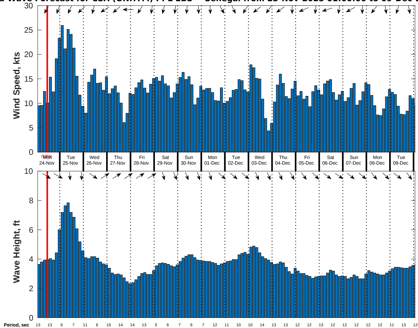
Wind & Wave Forecast for CSA (ONHYM) PPL EBS - Senegal from 23-Nov-2025 01:00:00 to 09-Dec-2025 01:00:00
