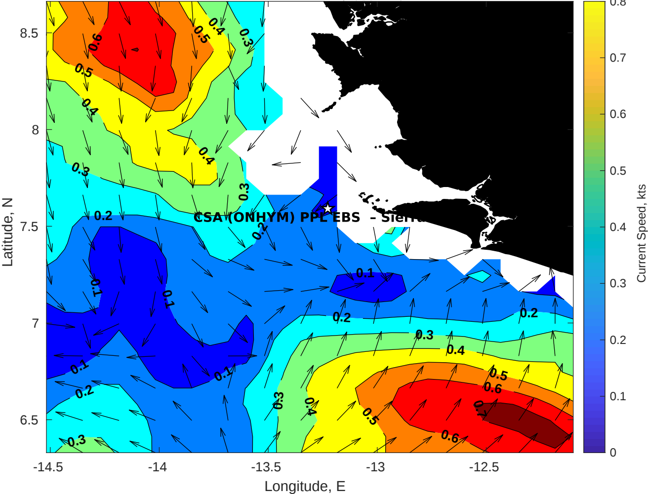
Surface Currents for CSA (ONHYM) PPL EBS - Sierra Leone at 22-Nov-2025 00:00:00
