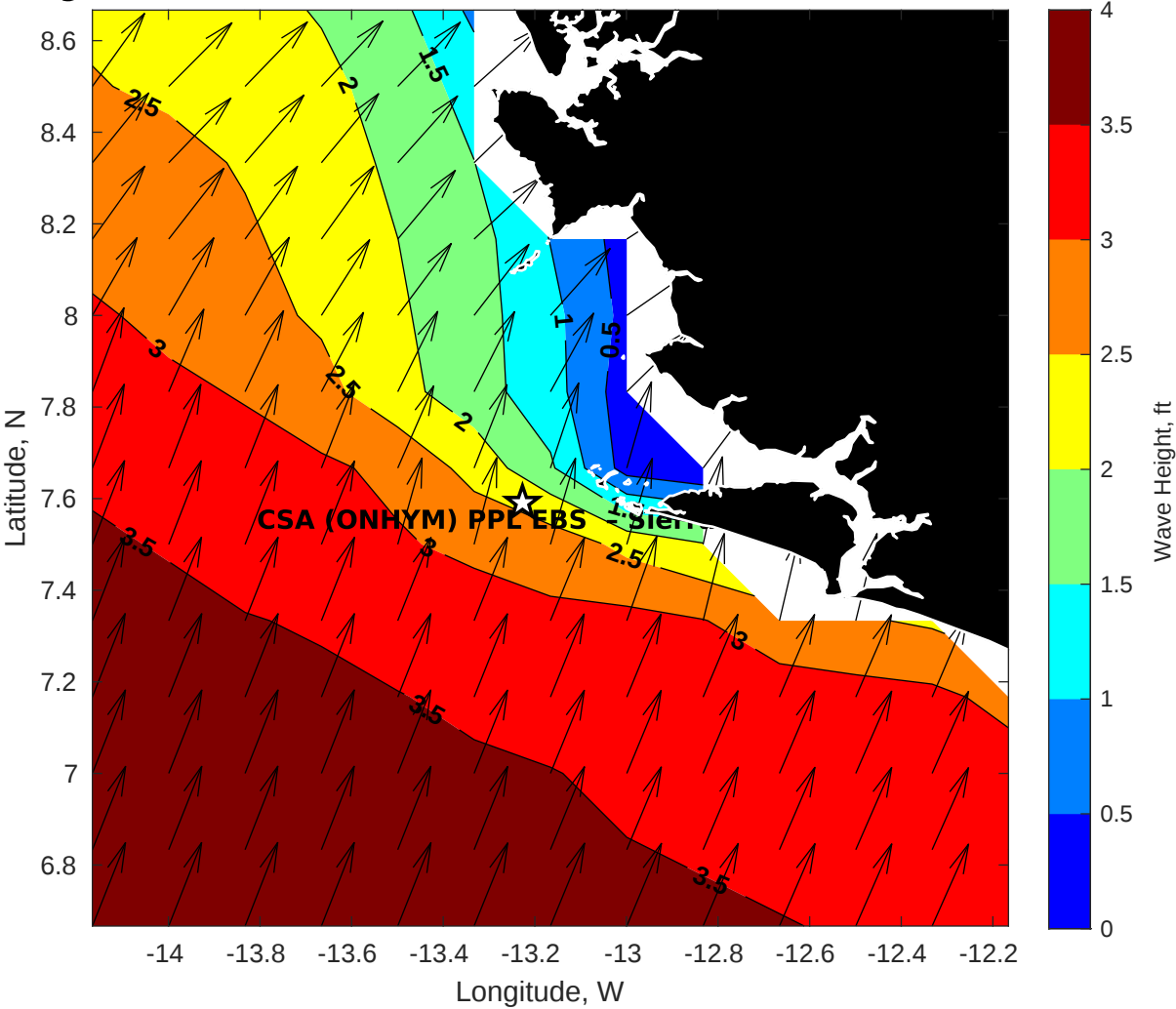
GFS Wave Height (ft) for CSA (ONHYM) PPL EBS - Sierra Leone at 23-Nov-2025 09:00:00
