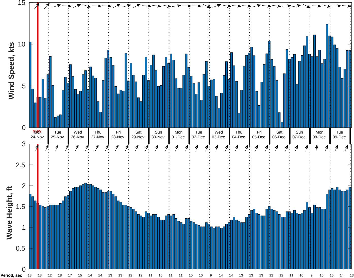
Wind & Wave Forecast for CSA (ONHYM) PPL EBS - Sierra Leone from 23-Nov-2025 01:00:00 to 09-Dec-2025 01:00:00
