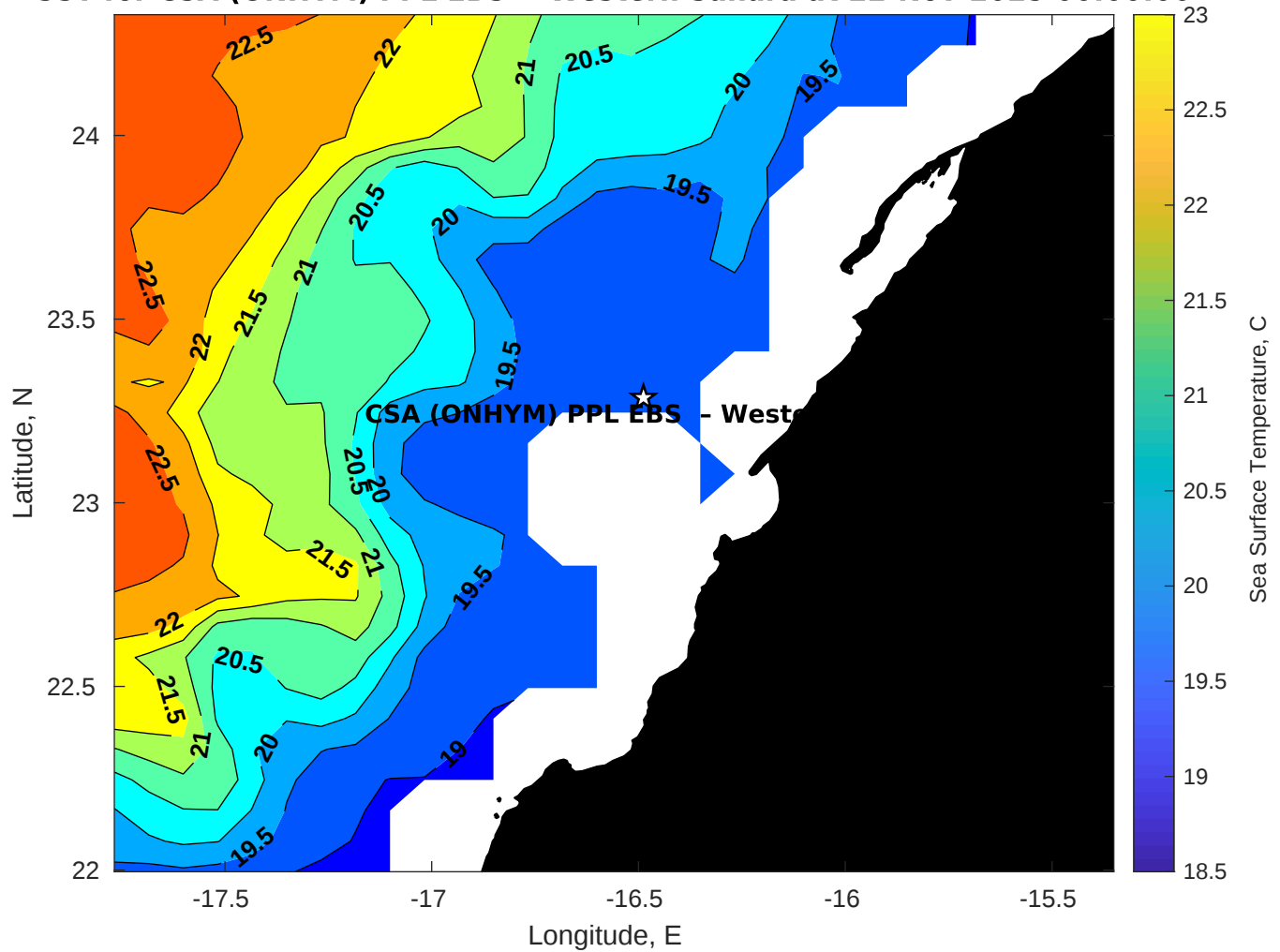
SST for CSA (ONHYM) PPL EBS - Western Sahara at 22-Nov-2025 00:00:00
