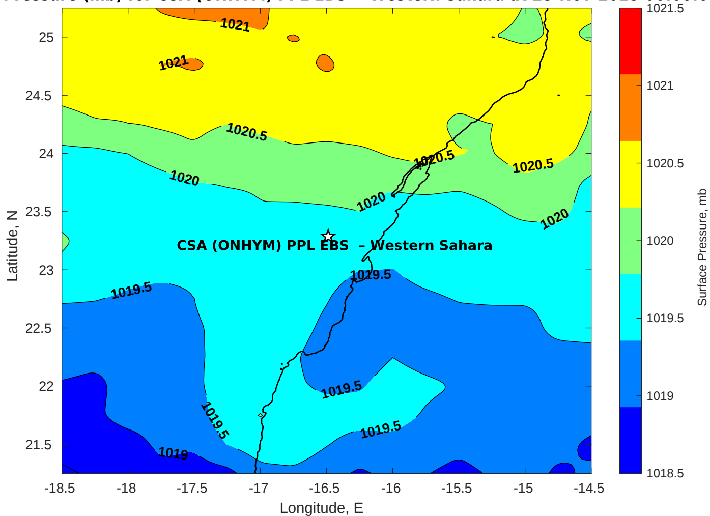
Surface Pressure (mb) for CSA (ONHYM) PPL EBS - Western Sahara at 25-Nov-2025 00:00:00
