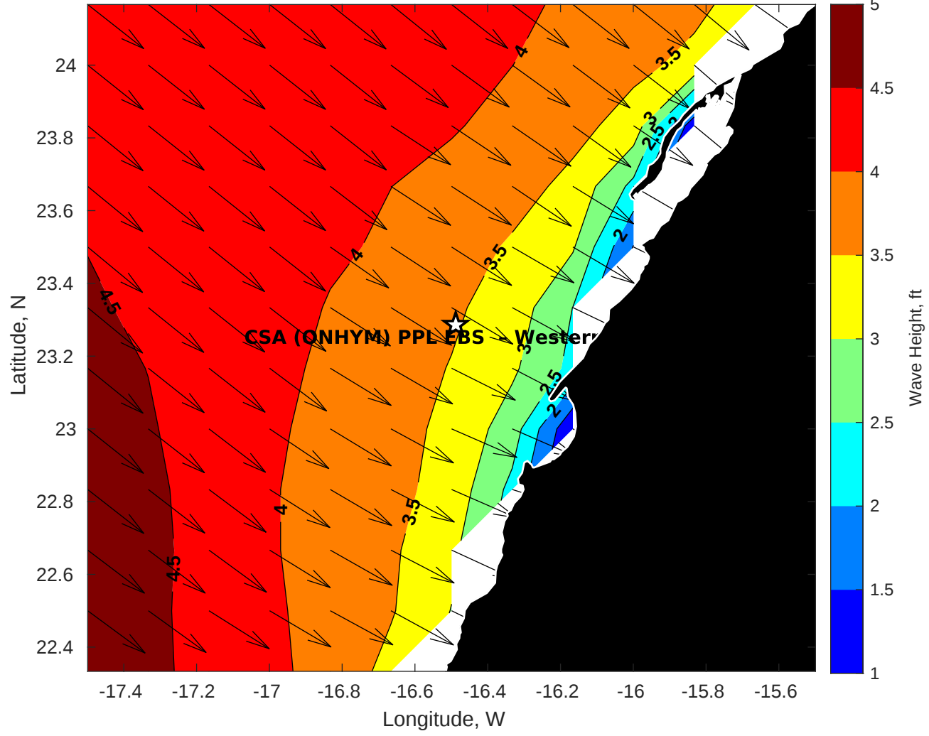
GFS Wave Height (ft) for CSA (ONHYM) PPL EBS - Western Sahara at 23-Nov-2025 09:00:00
