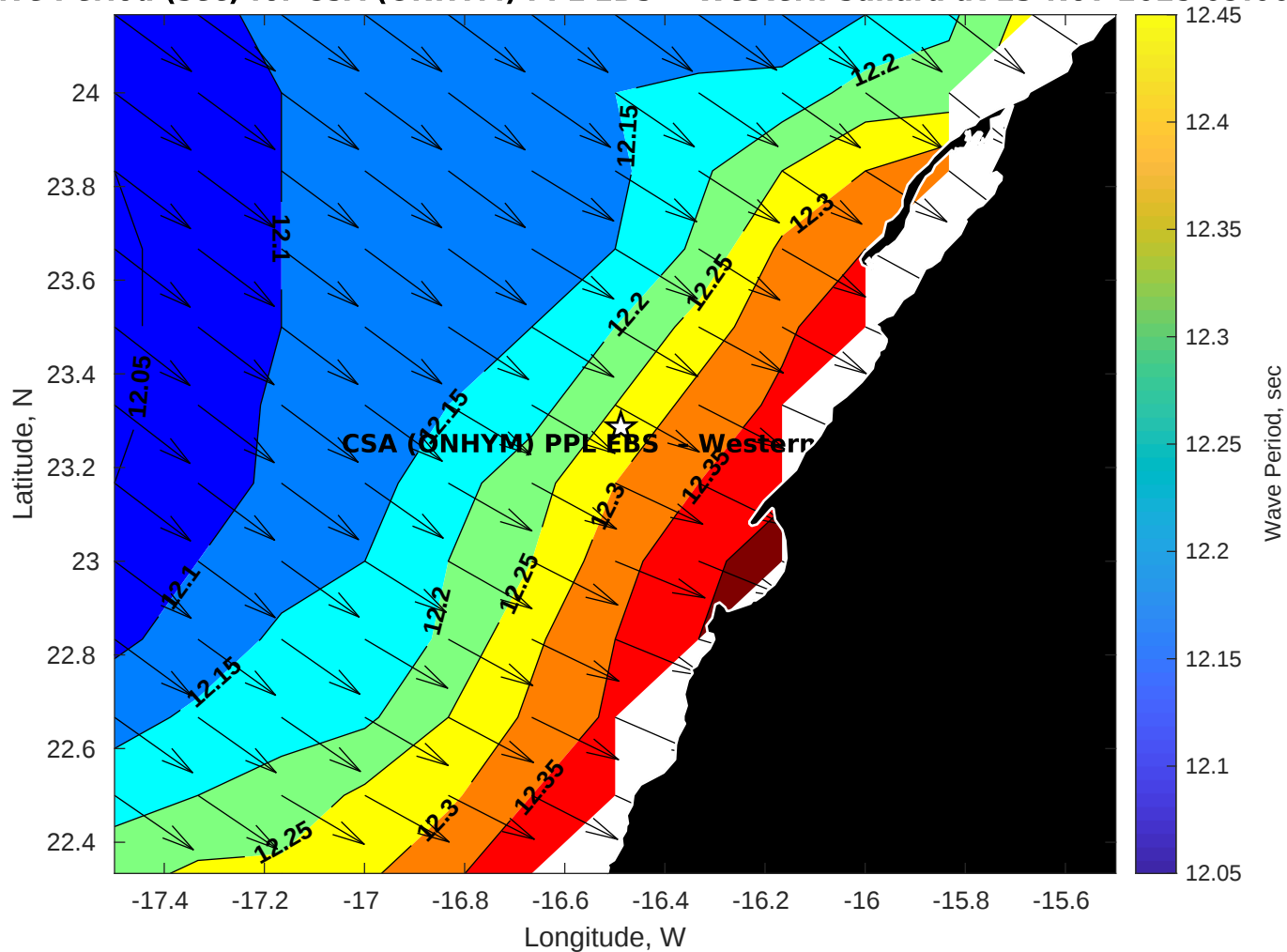
GFS Wave Period (sec) for CSA (ONHYM) PPL EBS - Western Sahara at 23-Nov-2025 09:00:00
