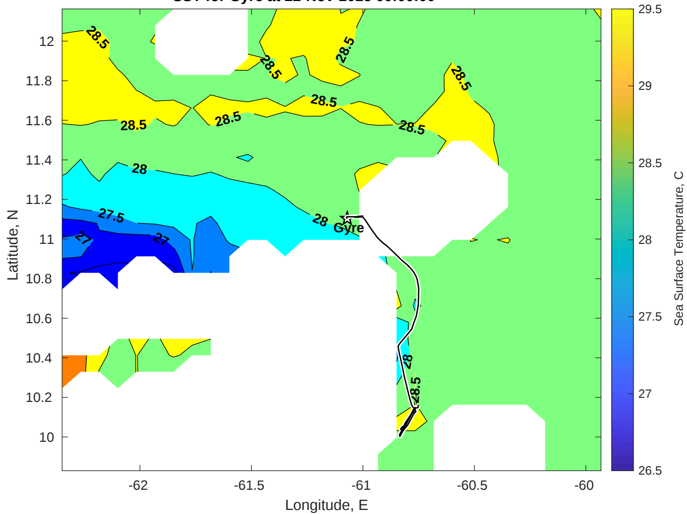
SST for Gyre at 22-Nov-2025 00:00:00
