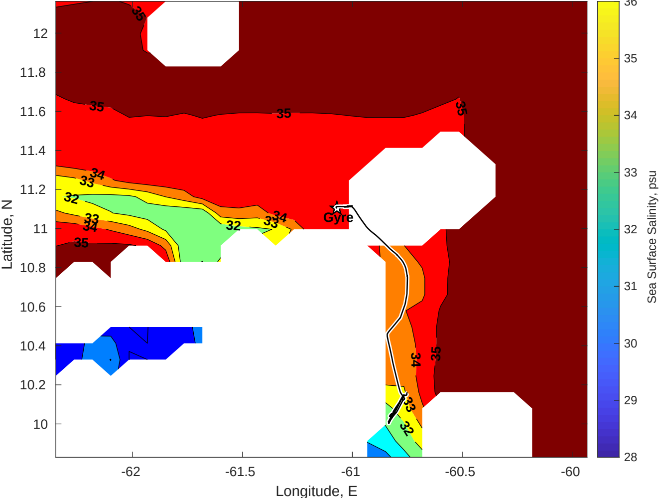
Surface Salinity for Gyre at 22-Nov-2025 00:00:00
