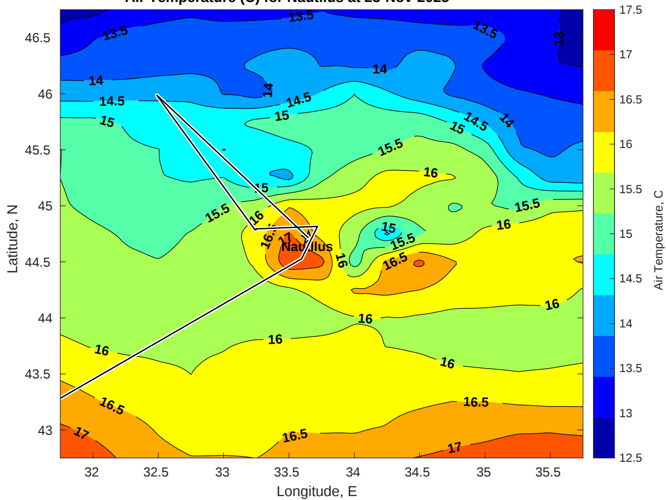
Air Temperature (C) for Nautilus at 23-Nov-2025
