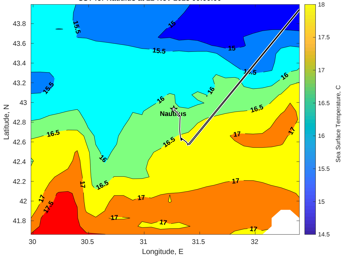
SST for Nautilus at 22-Nov-2025 00:00:00
