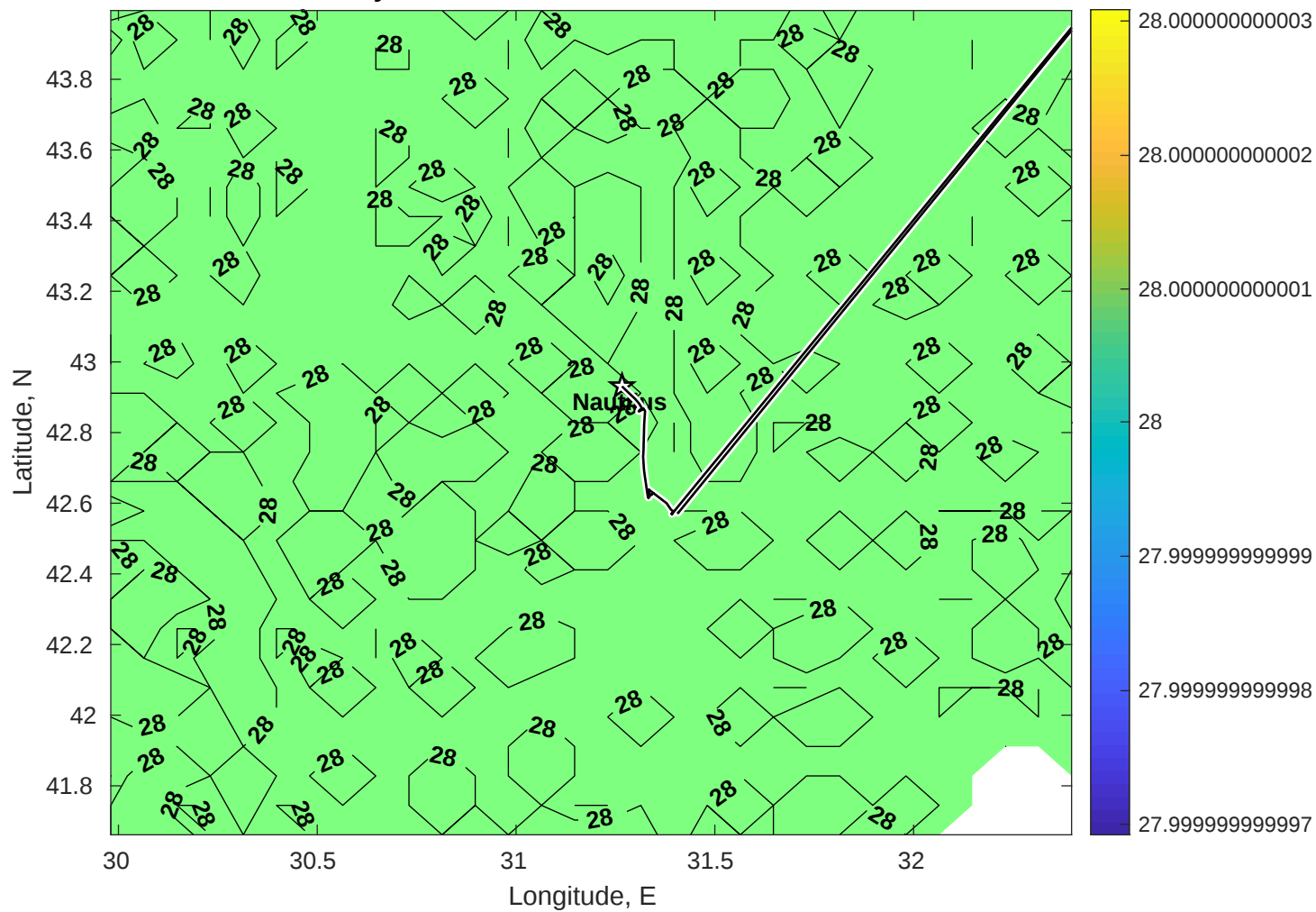
Surface Salinity for Nautilus at 22-Nov-2025 00:00:00
