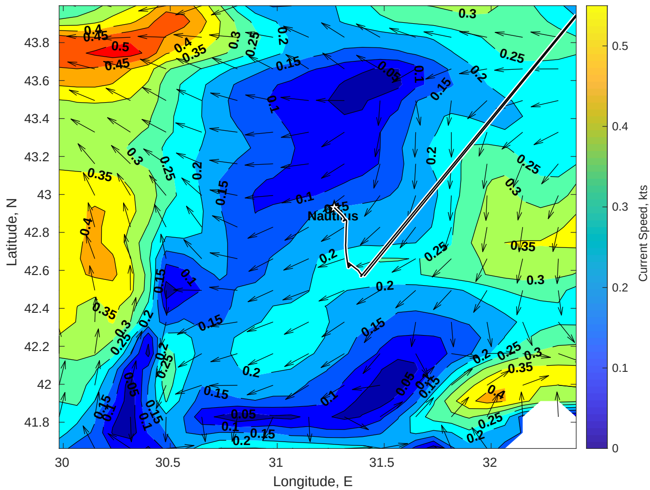
Surface Currents for Nautilus at 22-Nov-2025 00:00:00
