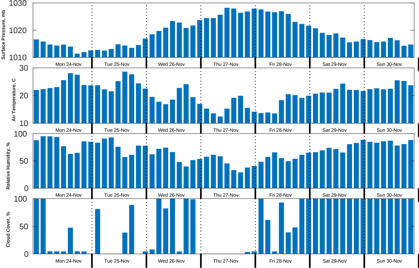
Met Forecast for Brooks McCall from 24-Nov-2025 00:00:00 to 01-Dec-2025 00:00:00
