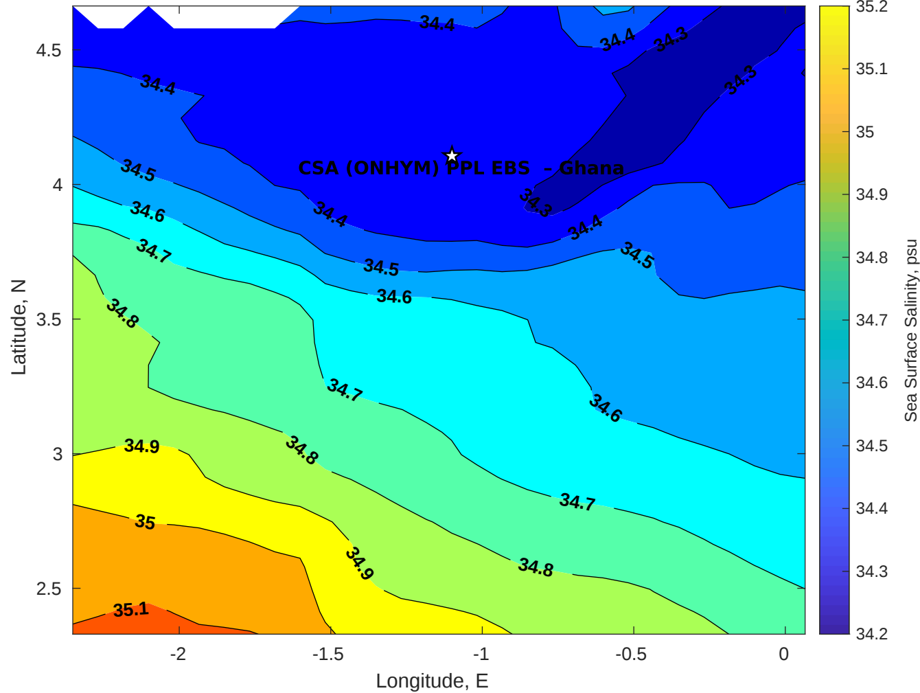
Surface Salinity for CSA (ONHYM) PPL EBS - Ghana at 23-Nov-2025 00:00:00
