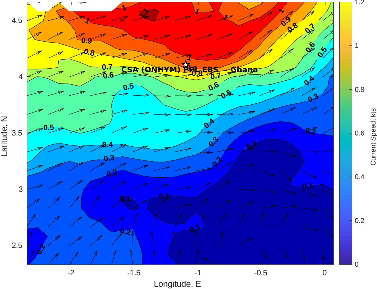
Surface Currents for CSA (ONHYM) PPL EBS - Ghana at 23-Nov-2025 00:00:00
