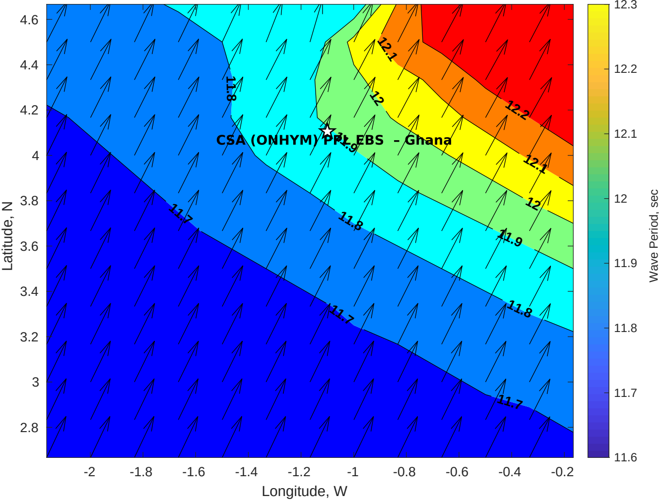
GFS Wave Period (sec) for CSA (ONHYM) PPL EBS - Ghana at 24-Nov-2025 09:00:00
