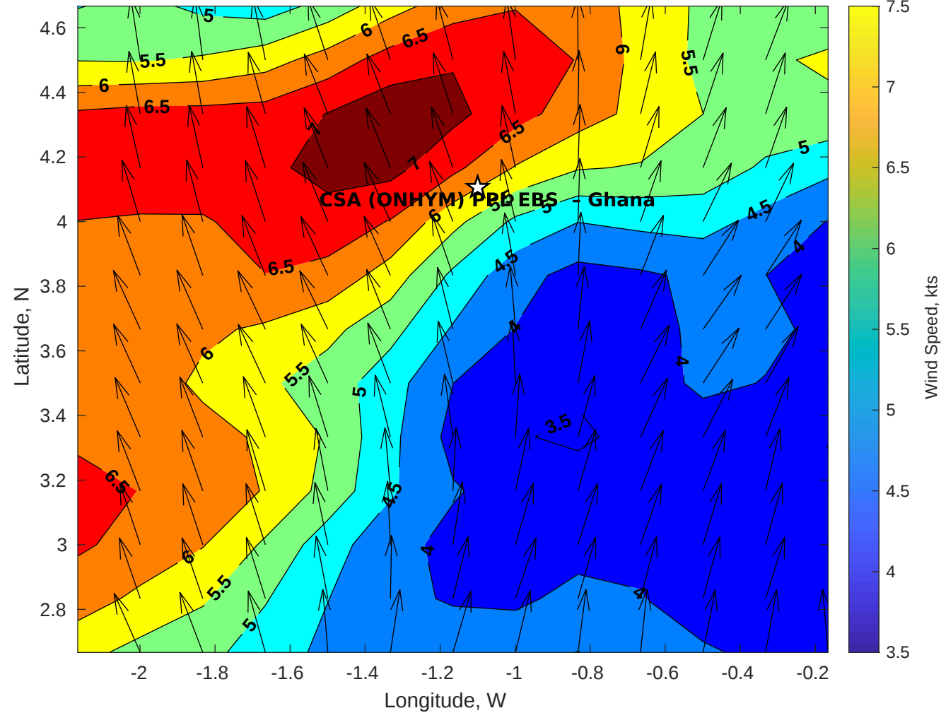
GFS Winds (kts) for CSA (ONHYM) PPL EBS - Ghana at 24-Nov-2025 09:00:00
