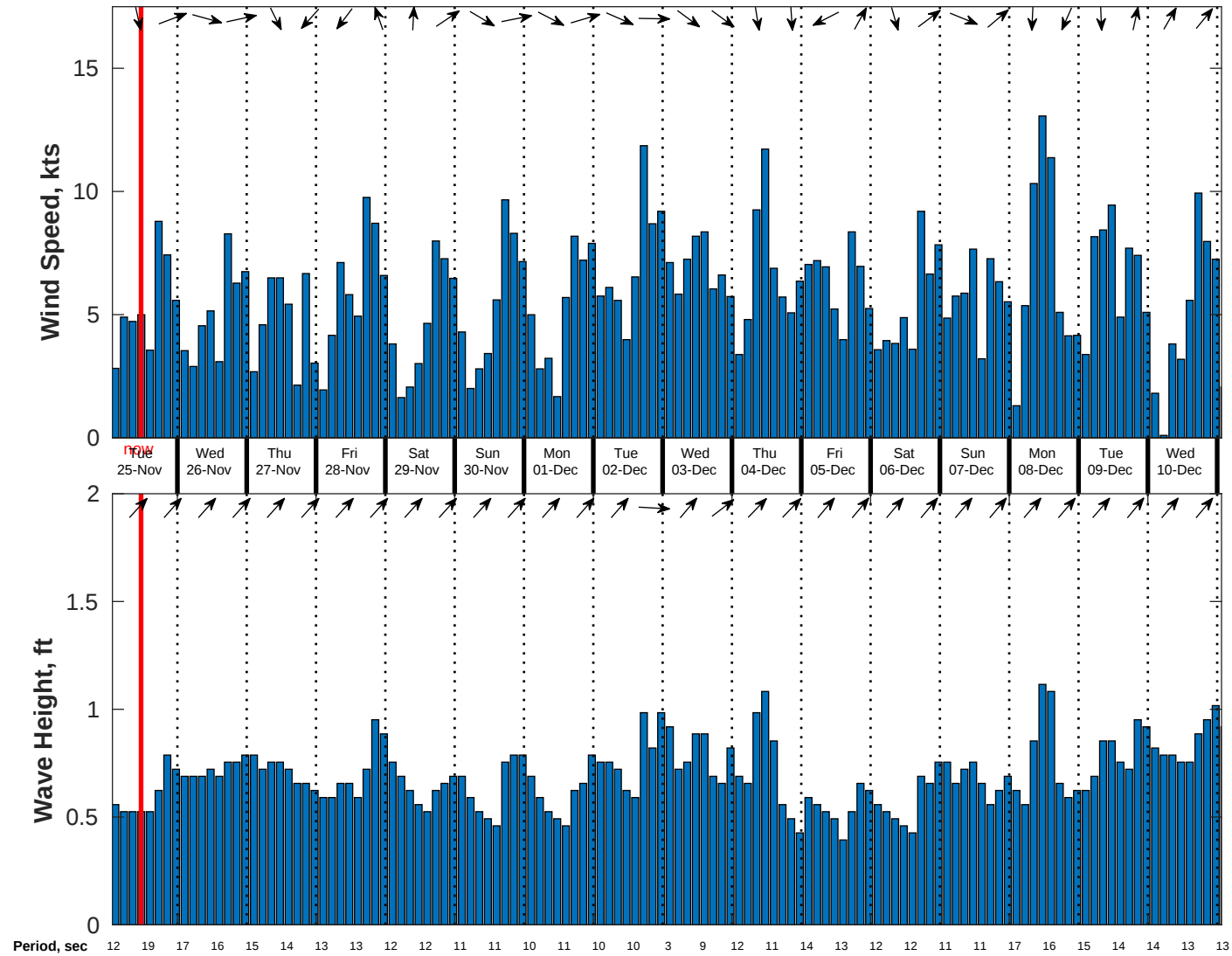
Wind & Wave Forecast for CSA (ONHYM) PPL EBS - Guinea from 24-Nov-2025 01:00:00 to 10-Dec-2025 01:00:00
