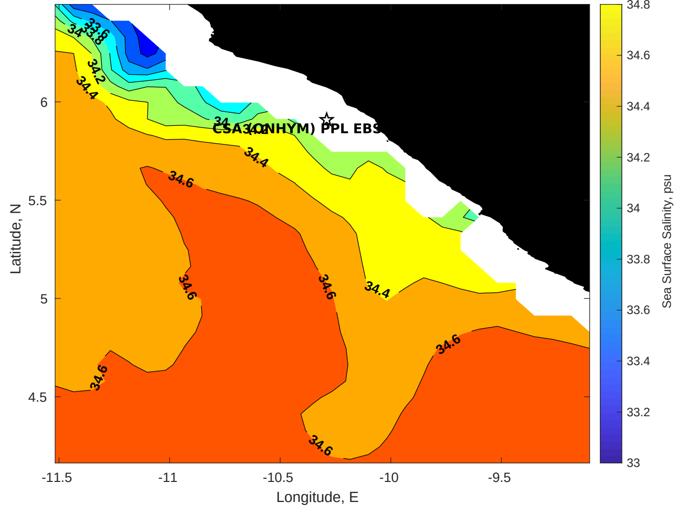
Surface Salinity for CSA (ONHYM) PPL EBS - Liberia at 23-Nov-2025 00:00:00
