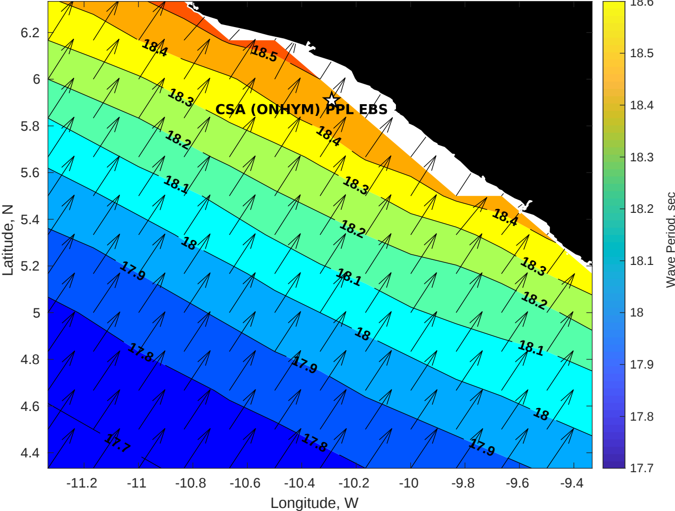
GFS Wave Period (sec) for CSA (ONHYM) PPL EBS - Liberia at 24-Nov-2025 09:00:00
