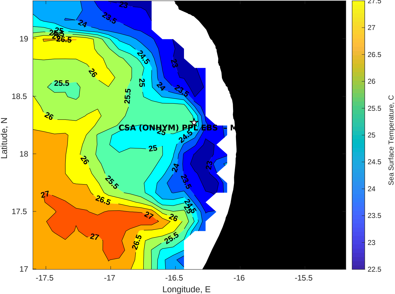
SST for CSA (ONHYM) PPL EBS - Mauritania at 23-Nov-2025 00:00:00
