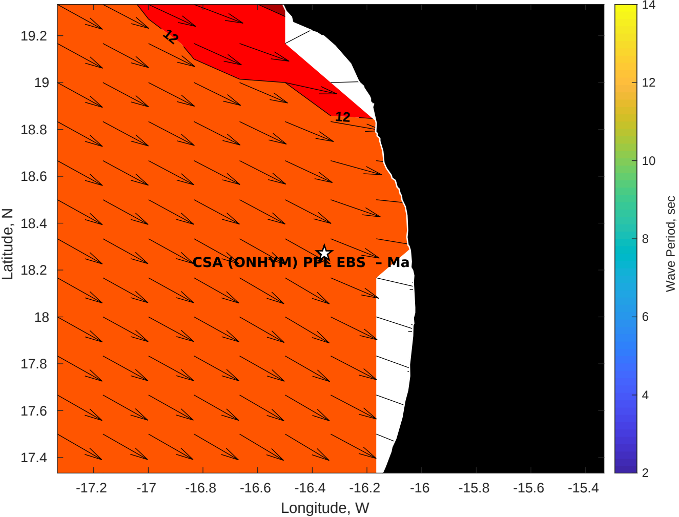
GFS Wave Period (sec) for CSA (ONHYM) PPL EBS - Mauritania at 24-Nov-2025 09:00:00
