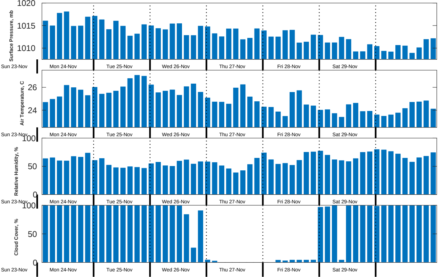
Met Forecast for CSA (ONHYM) PPL EBS - Mauritania from 24-Nov-2025 00:00:00 to 01-Dec-2025 00:00:00
