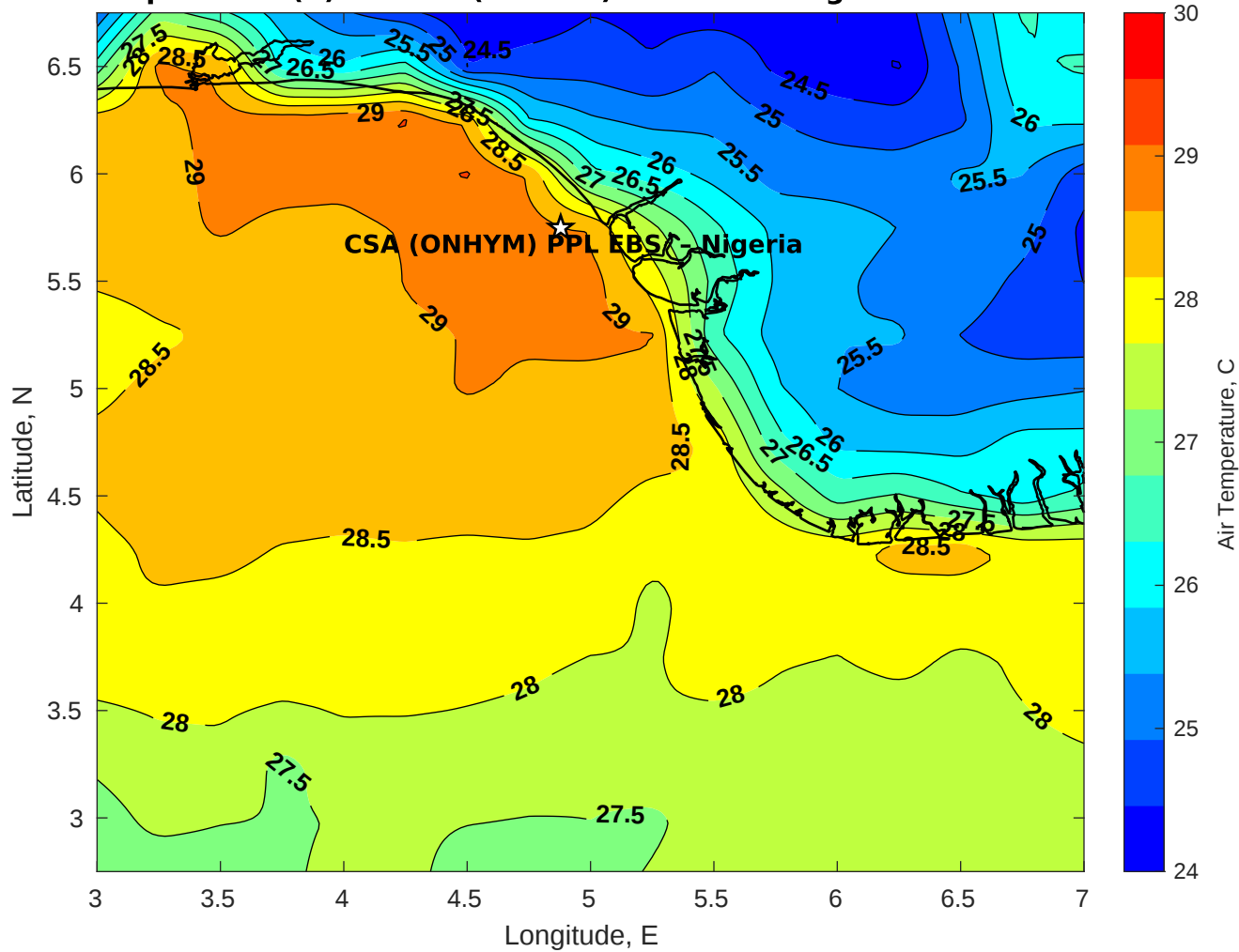
Air Temperature (C) for CSA (ONHYM) PPL EBS - Nigeria at 24-Nov-2025
