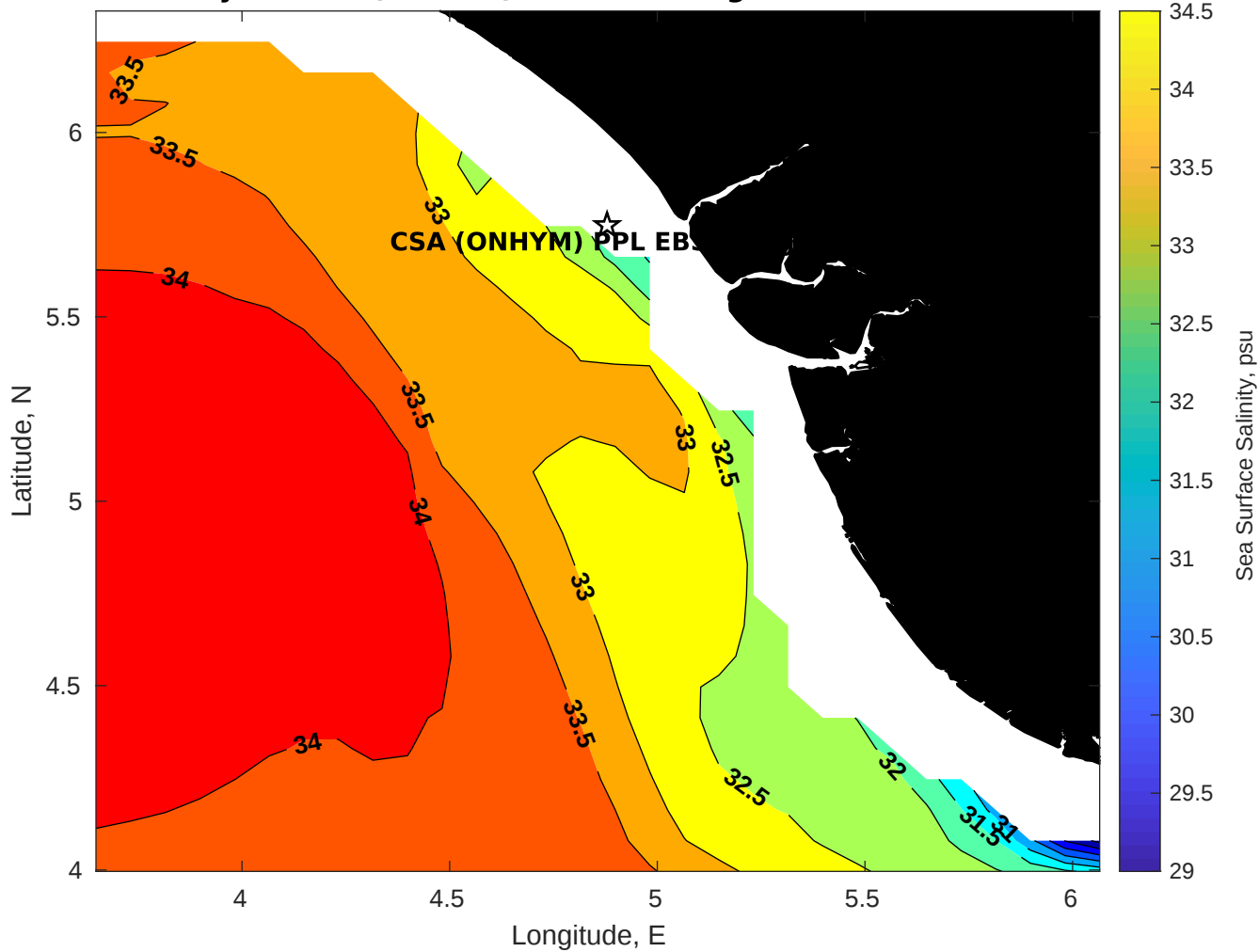
Surface Salinity for CSA (ONHYM) PPL EBS - Nigeria at 23-Nov-2025 00:00:00
