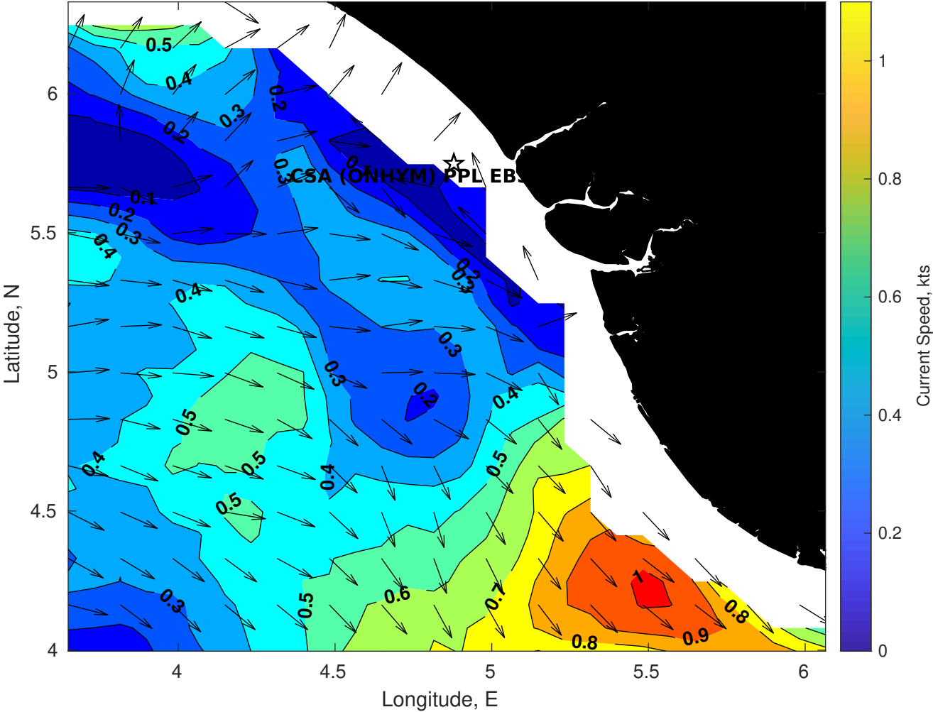
Surface Currents for CSA (ONHYM) PPL EBS - Nigeria at 23-Nov-2025 00:00:00
