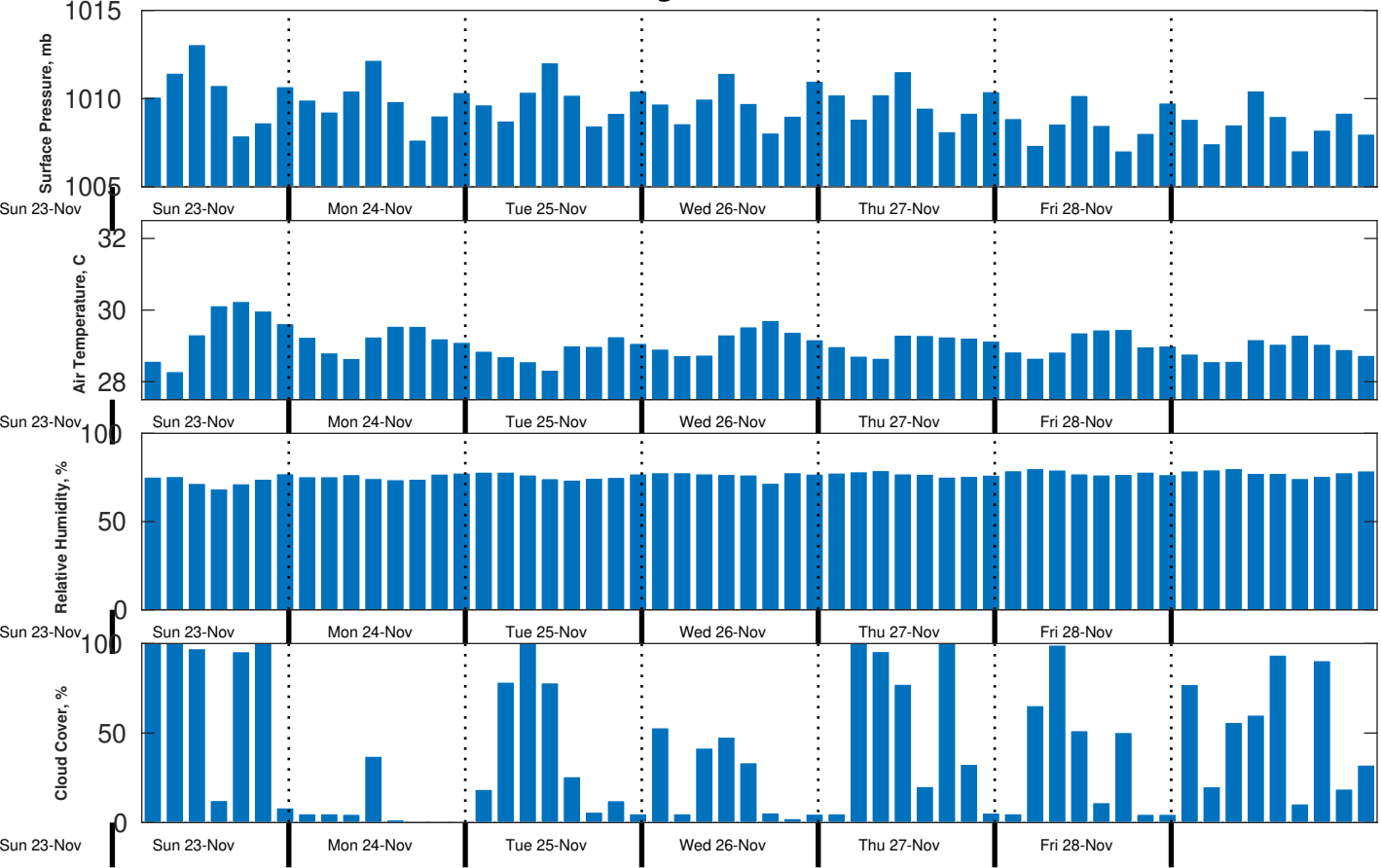
Met Forecast for CSA (ONHYM) PPL EBS - Nigeria from 24-Nov-2025 00:00:00 to 01-Dec-2025 00:00:00
