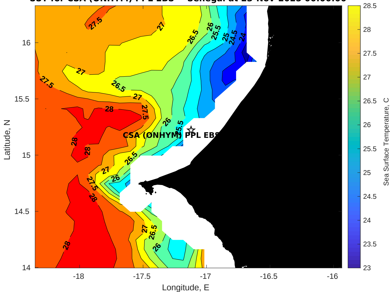
SST for CSA (ONHYM) PPL EBS - Senegal at 23-Nov-2025 00:00:00
