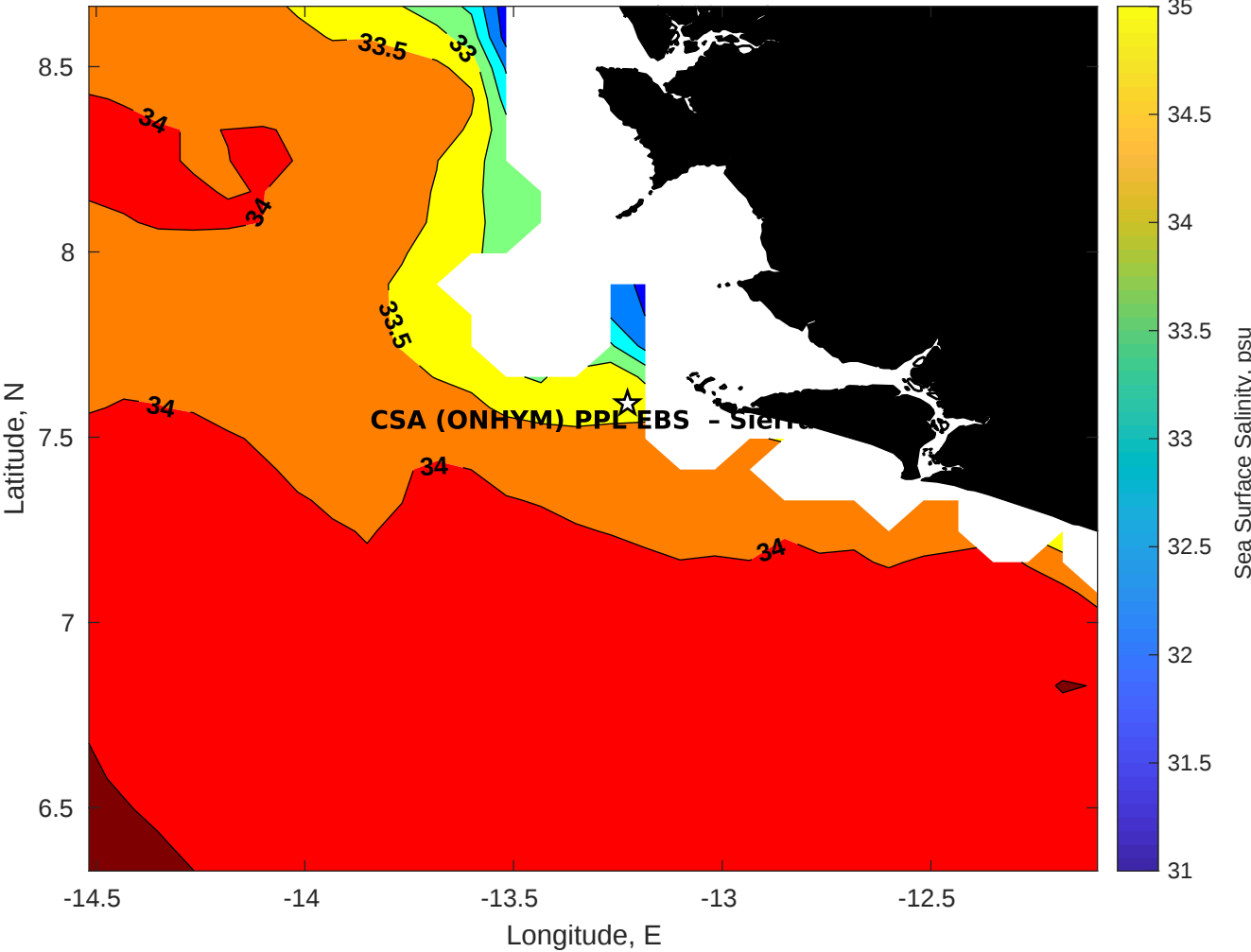
Surface Salinity for CSA (ONHYM) PPL EBS - Sierra Leone at 23-Nov-2025 00:00:00
