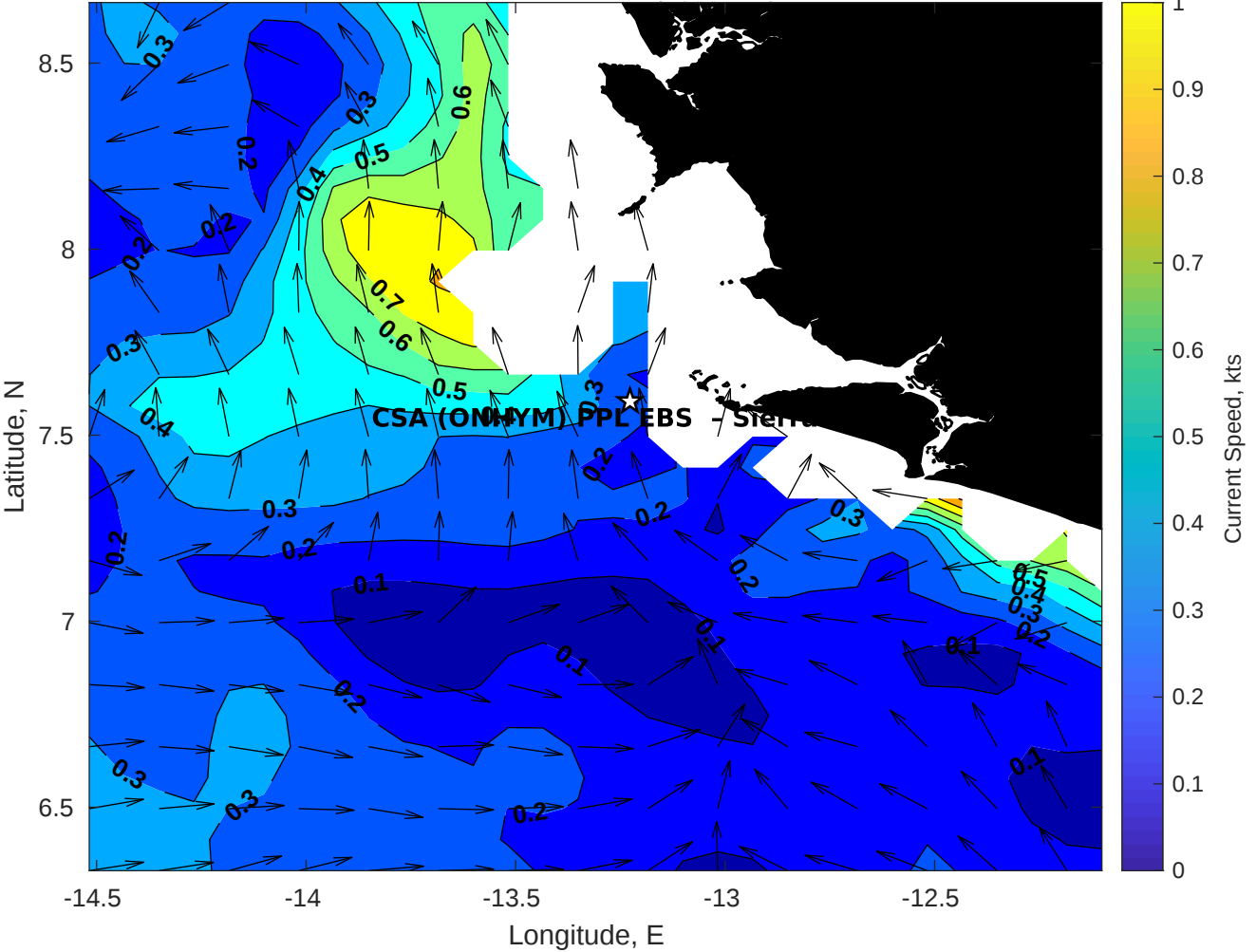
Surface Currents for CSA (ONHYM) PPL EBS - Sierra Leone at 23-Nov-2025 00:00:00
