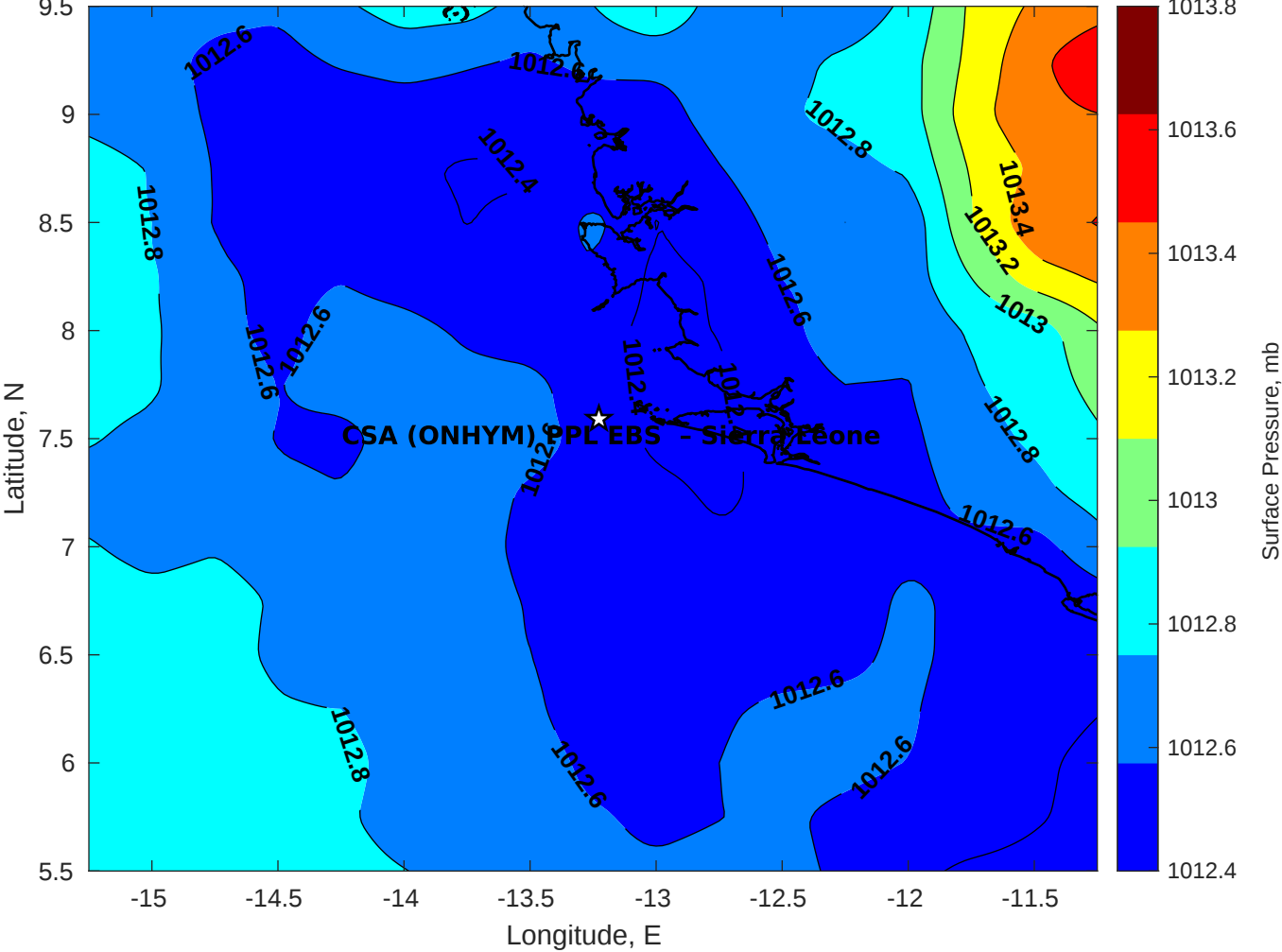
Surface Pressure (mb) for CSA (ONHYM) PPL EBS - Sierra Leone at 24-Nov-2025 00:00:00
