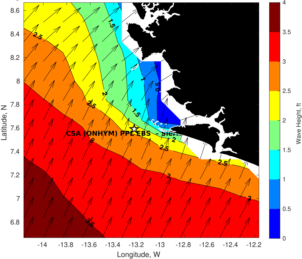
GFS Wave Height (ft) for CSA (ONHYM) PPL EBS - Sierra Leone at 24-Nov-2025 09:00:00
