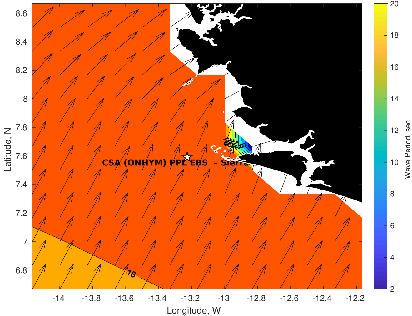
GFS Wave Period (sec) for CSA (ONHYM) PPL EBS - Sierra Leone at 24-Nov-2025 09:00:00
