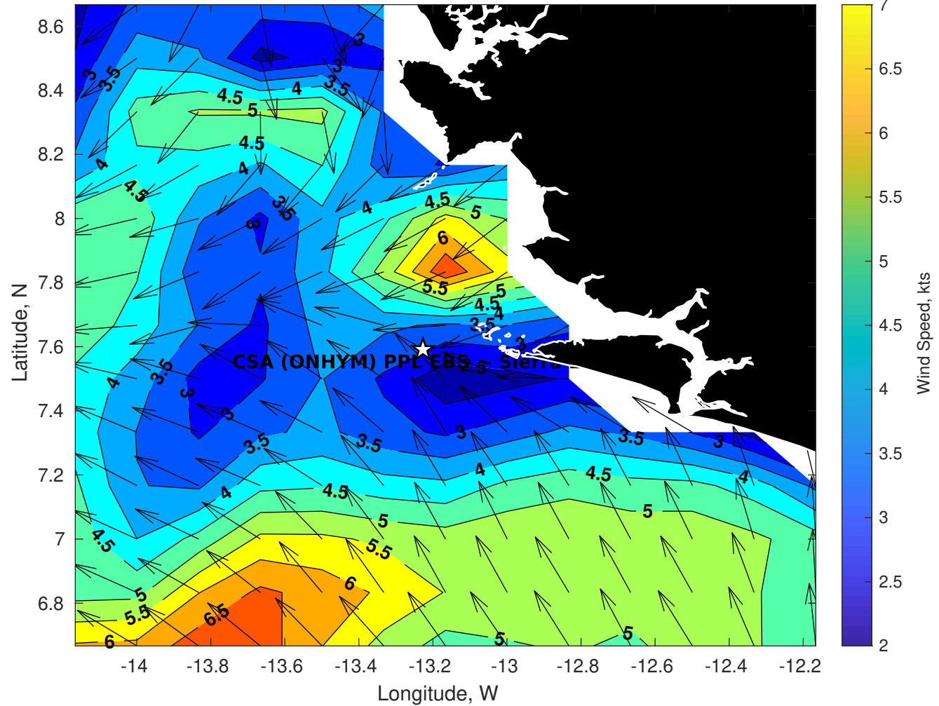
GFS Winds (kts) for CSA (ONHYM) PPL EBS - Sierra Leone at 24-Nov-2025 09:00:00
