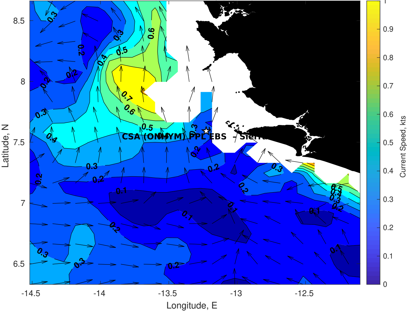
Surface Currents for CSA (ONHYM) PPL EBS - Sierra Leone at 23-Nov-2025 00:00:00
