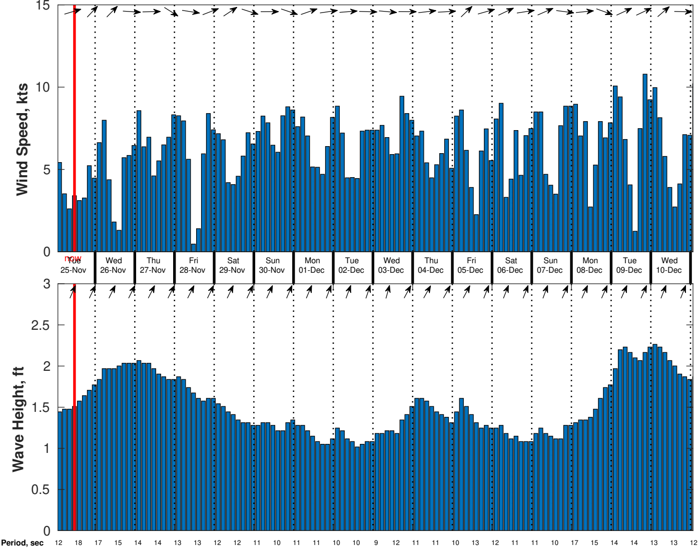
Wind & Wave Forecast for CSA (ONHYM) PPL EBS - Sierra Leone from 24-Nov-2025 01:00:00 to 10-Dec-2025 01:00:00
