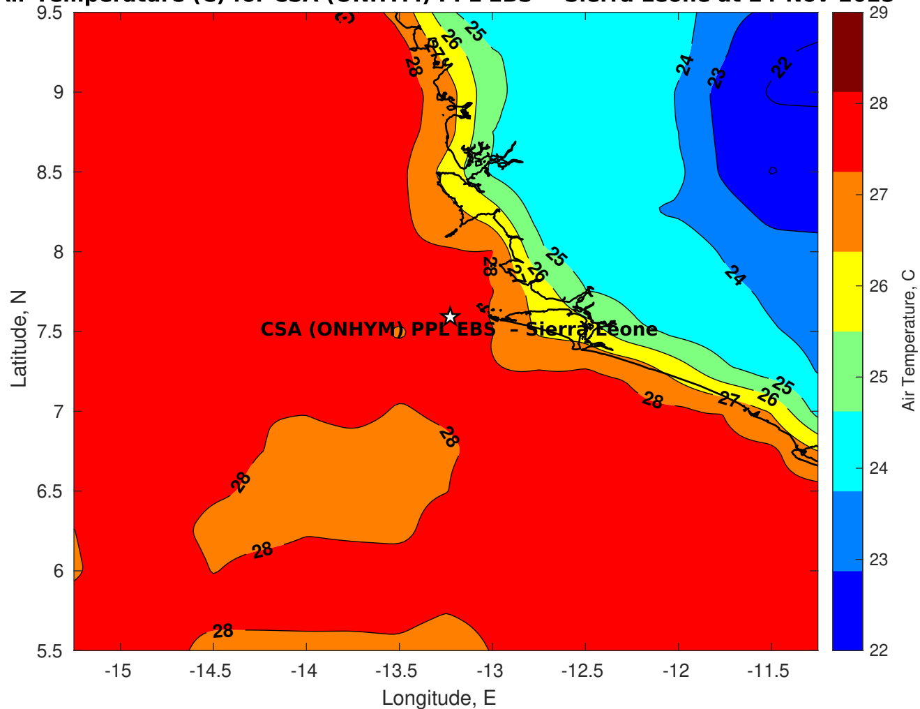
Air Temperature (C) for CSA (ONHYM) PPL EBS - Sierra Leone at 24-Nov-2025
