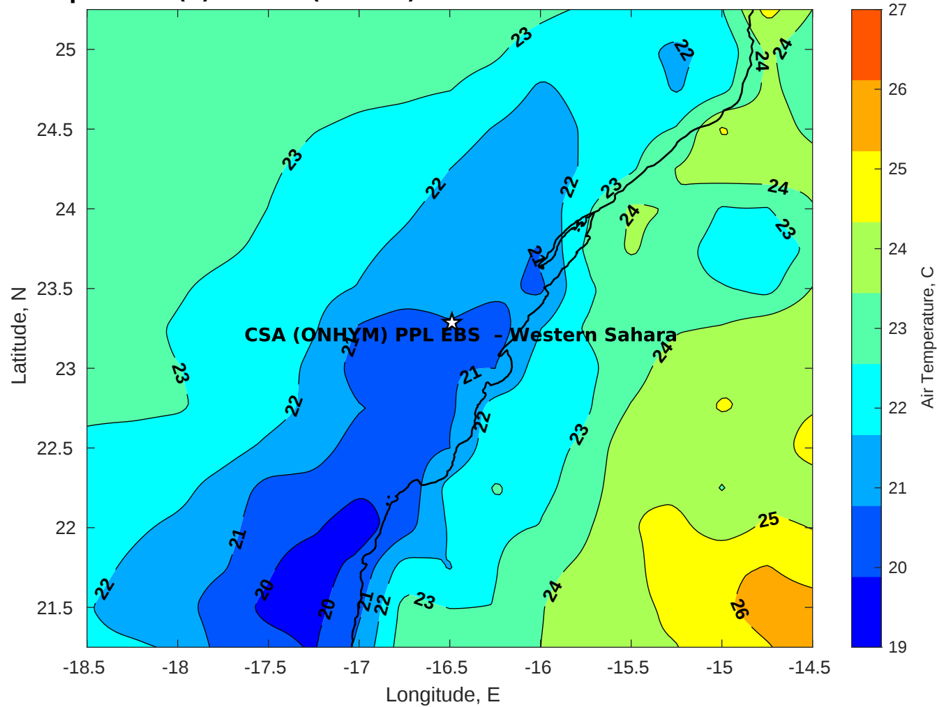
Air Temperature (C) for CSA (ONHYM) PPL EBS - Western Sahara at 24-Nov-2025
