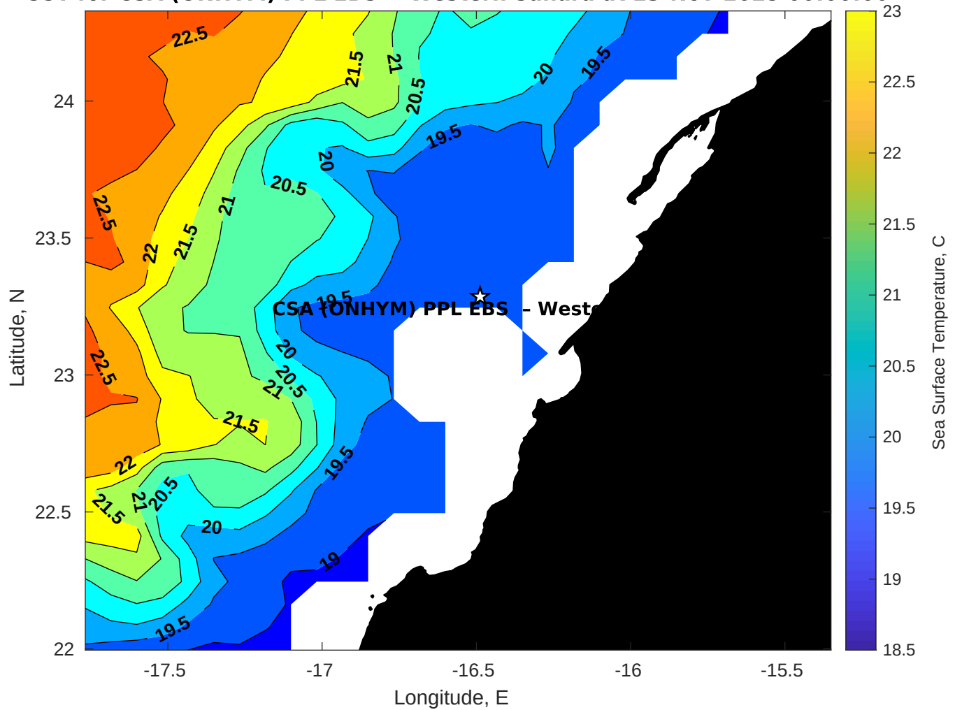
SST for CSA (ONHYM) PPL EBS - Western Sahara at 23-Nov-2025 00:00:00
