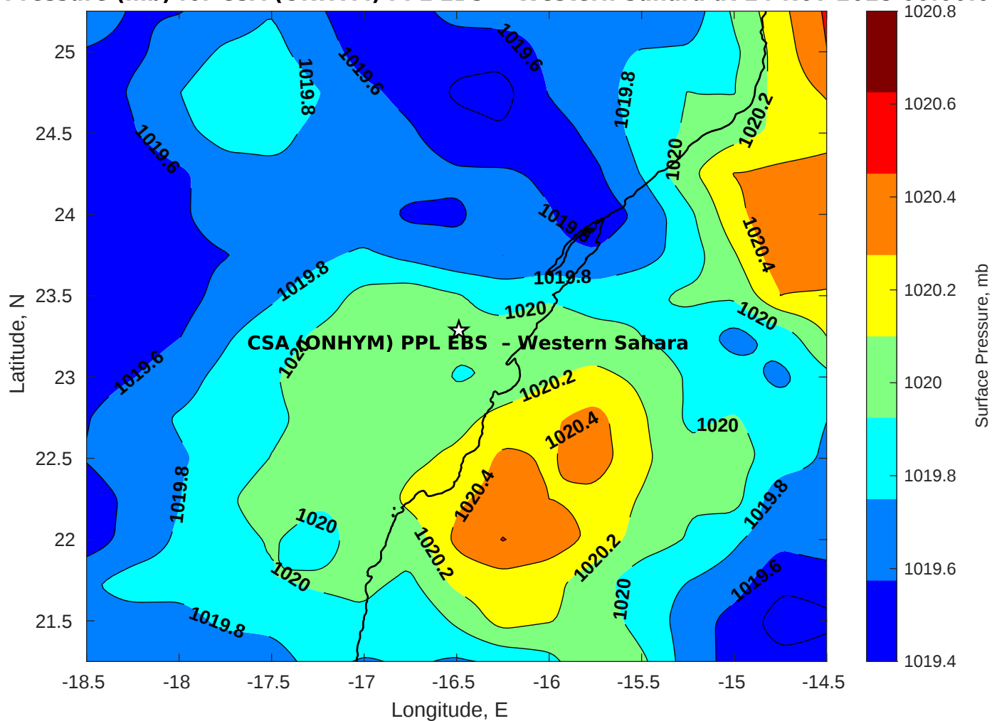
Surface Pressure (mb) for CSA (ONHYM) PPL EBS - Western Sahara at 24-Nov-2025 00:00:00
