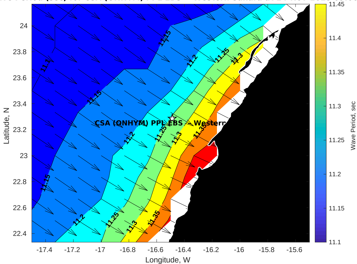
GFS Wave Period (sec) for CSA (ONHYM) PPL EBS - Western Sahara at 24-Nov-2025 09:00:00
