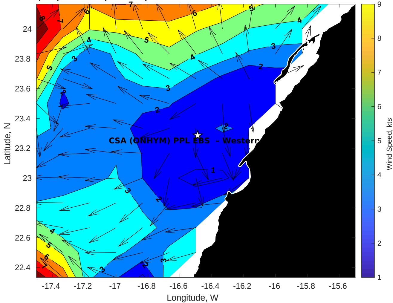
GFS Winds (kts) for CSA (ONHYM) PPL EBS - Western Sahara at 24-Nov-2025 09:00:00
