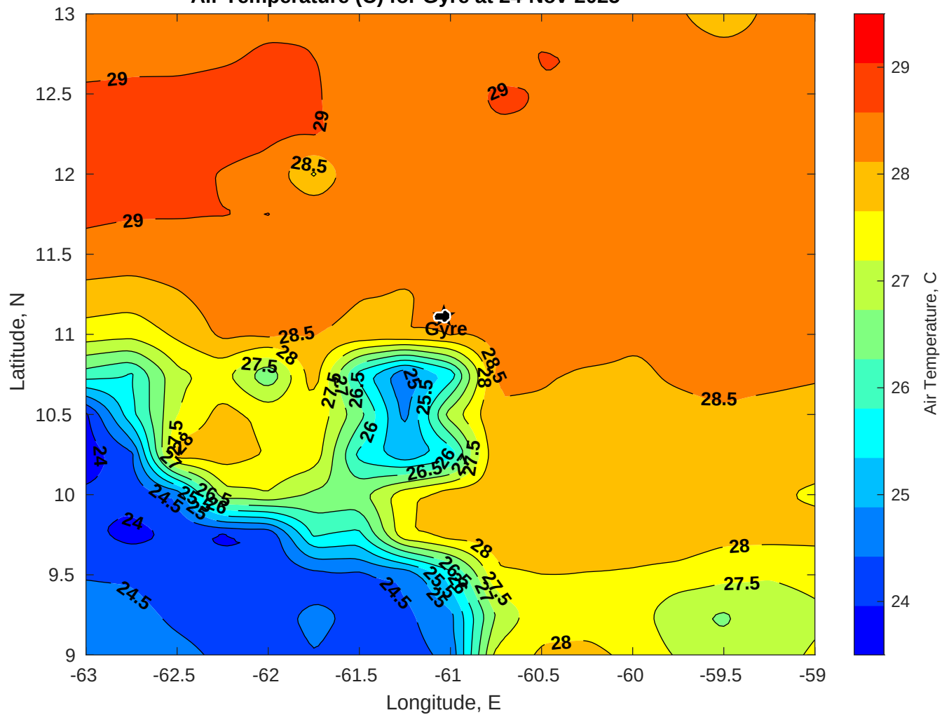
Air Temperature (C) for Gyre at 24-Nov-2025
