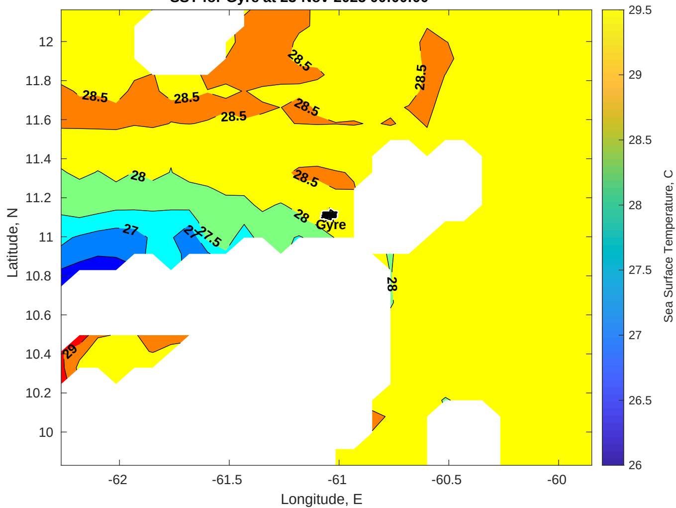
SST for Gyre at 23-Nov-2025 00:00:00
