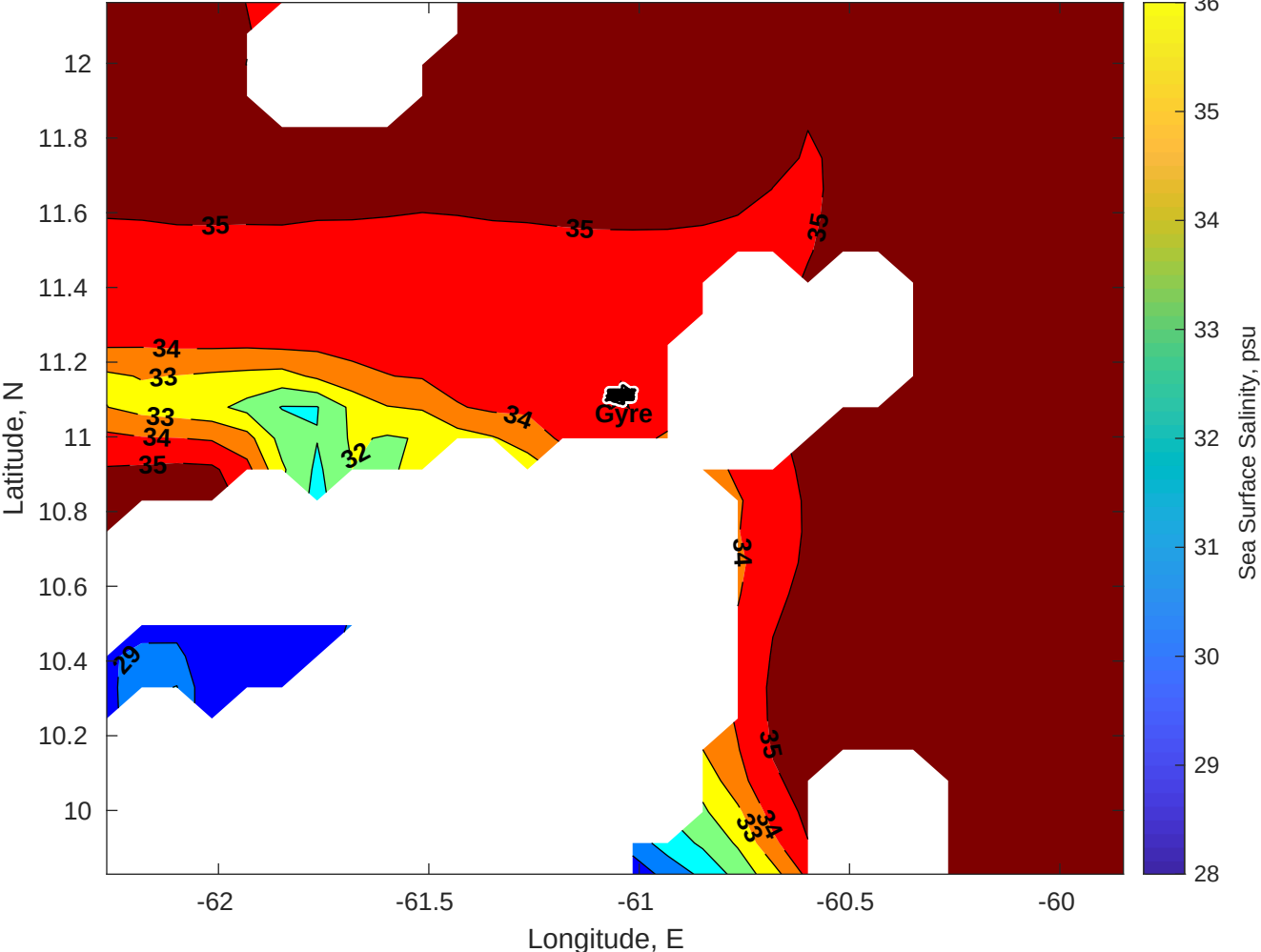
Surface Salinity for Gyre at 23-Nov-2025 00:00:00
