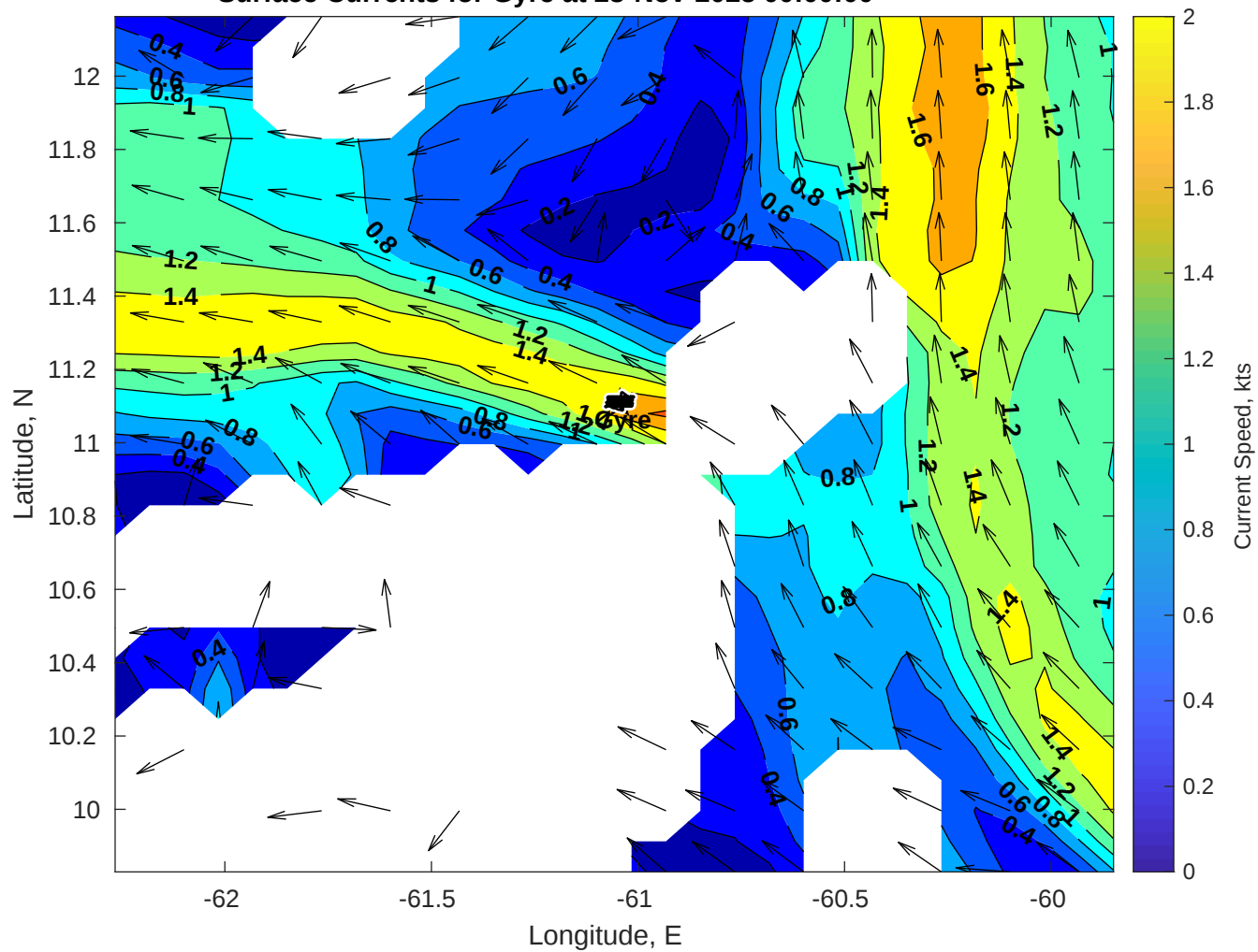
Surface Currents for Gyre at 23-Nov-2025 00:00:00
