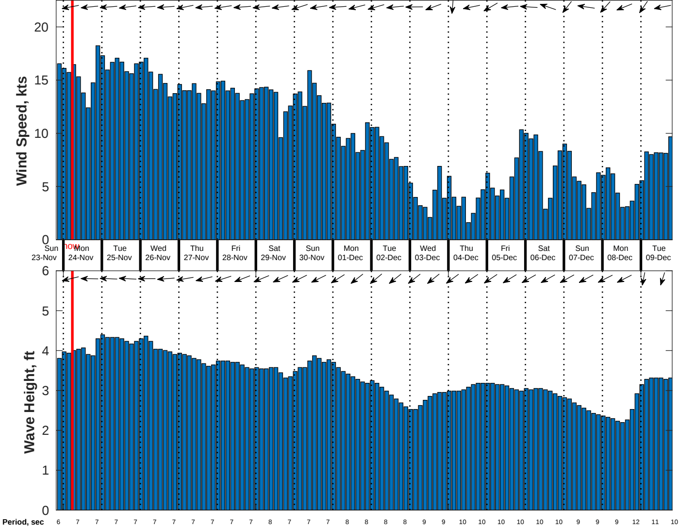
Wind & Wave Forecast for Gyre from 23-Nov-2025 20:00:00 to 09-Dec-2025 20:00:00
