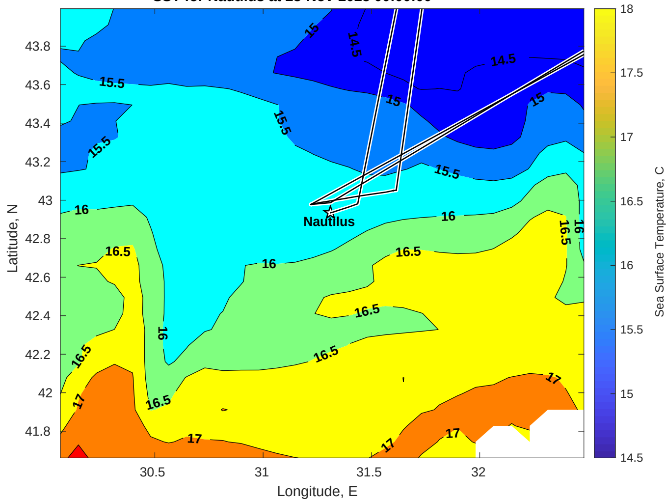
SST for Nautilus at 23-Nov-2025 00:00:00
