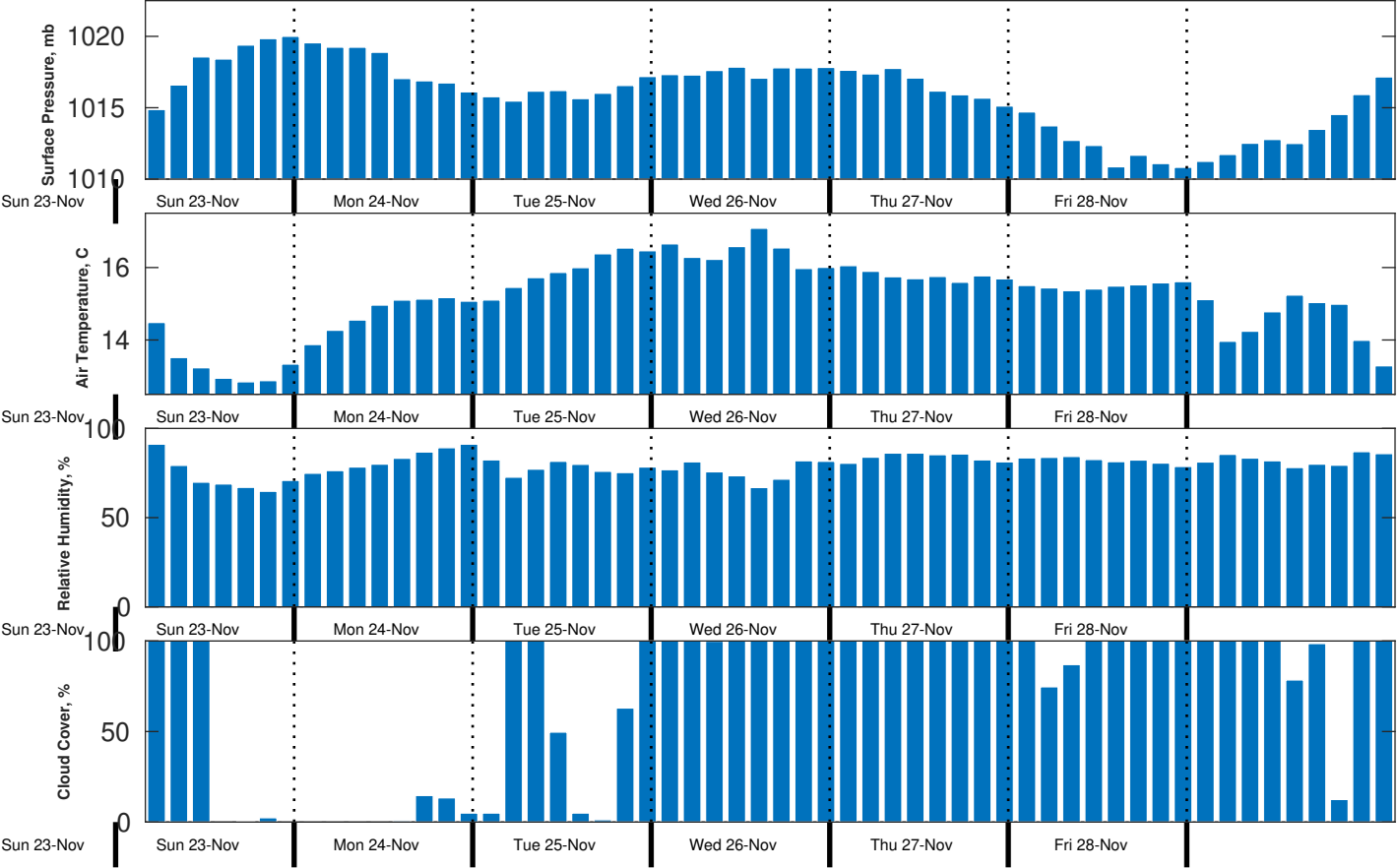
Met Forecast for Nautilus from 24-Nov-2025 00:00:00 to 01-Dec-2025 00:00:00
