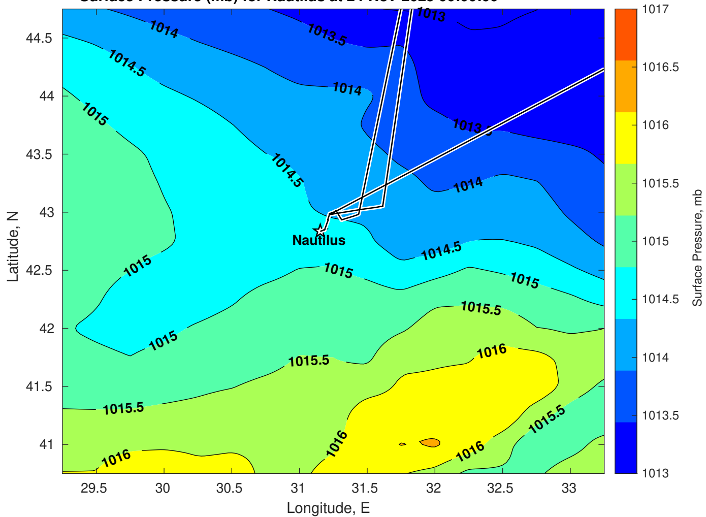
Surface Pressure (mb) for Nautilus at 24-Nov-2025 00:00:00
