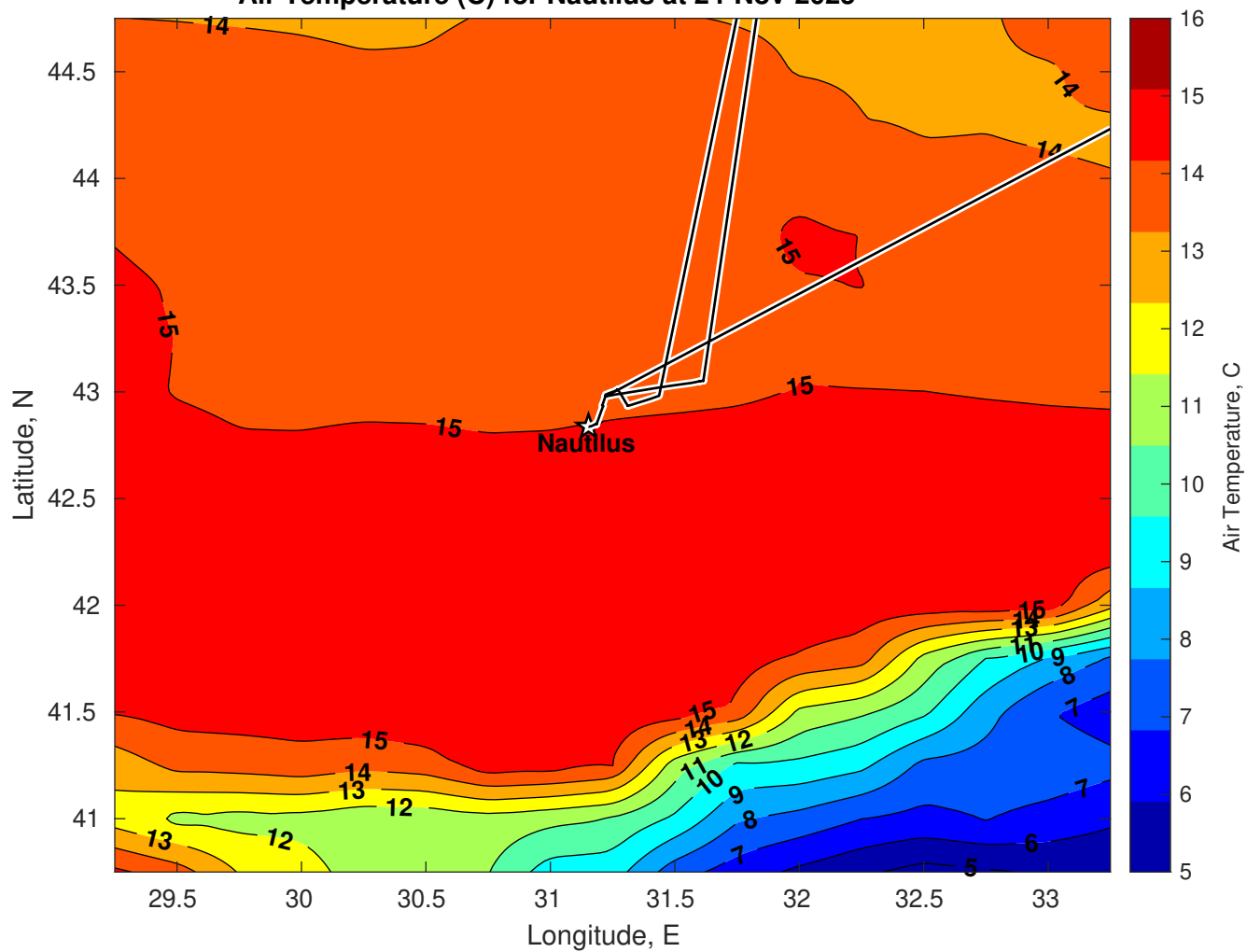
Air Temperature (C) for Nautilus at 24-Nov-2025
