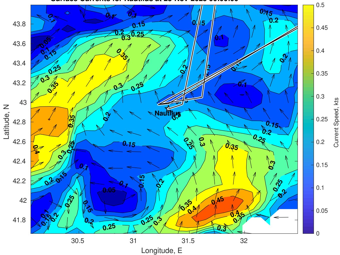
Surface Currents for Nautilus at 23-Nov-2025 00:00:00
