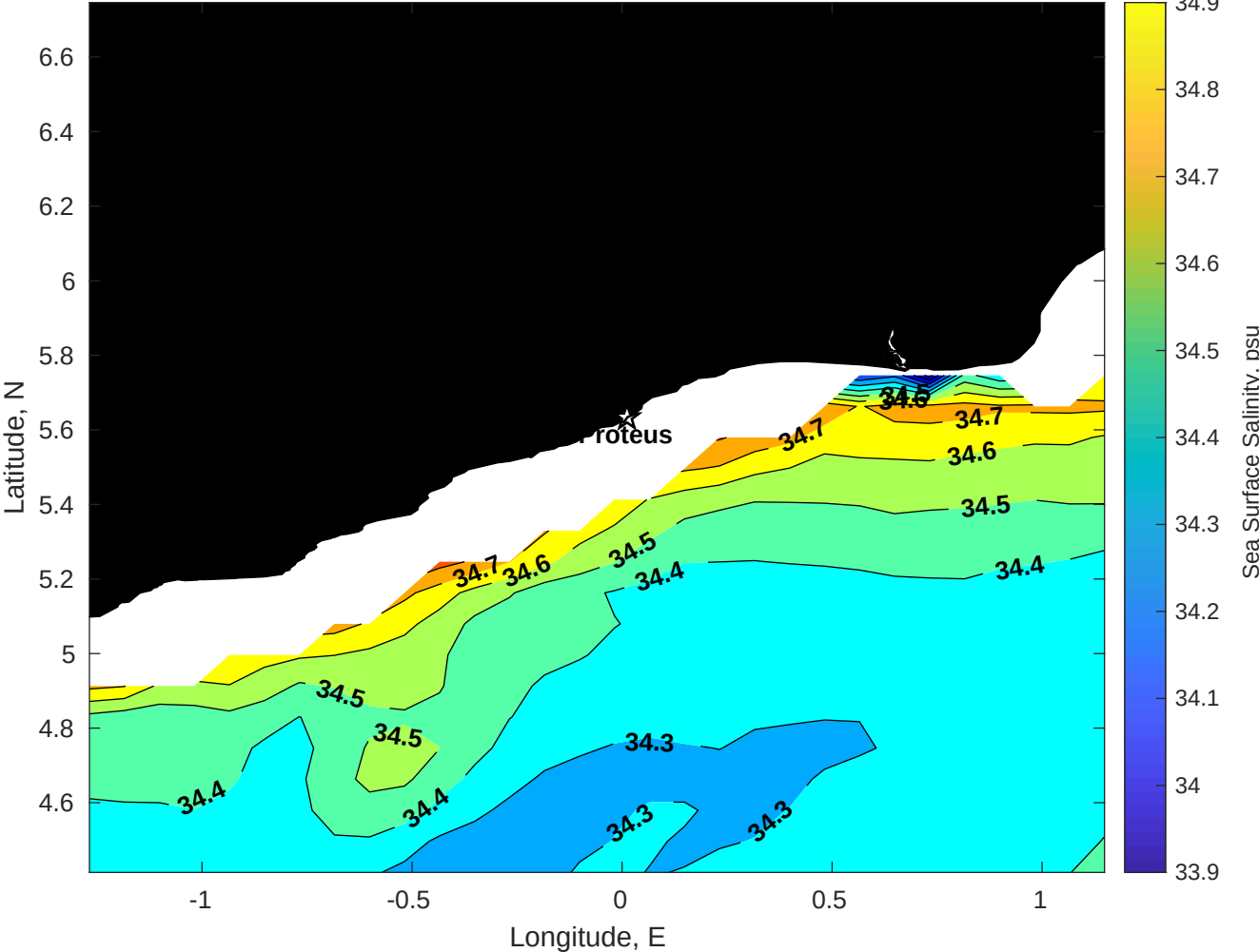
Surface Salinity for Proteus at 23-Nov-2025 00:00:00
