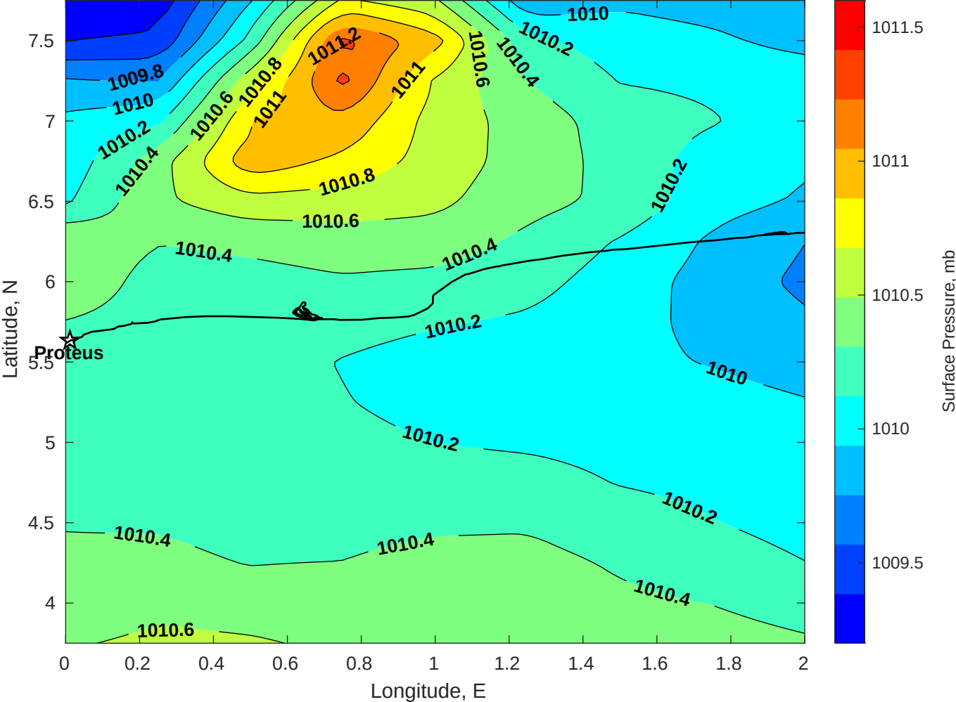
Surface Pressure (mb) for Proteus at 26-Nov-2025 00:00:00
