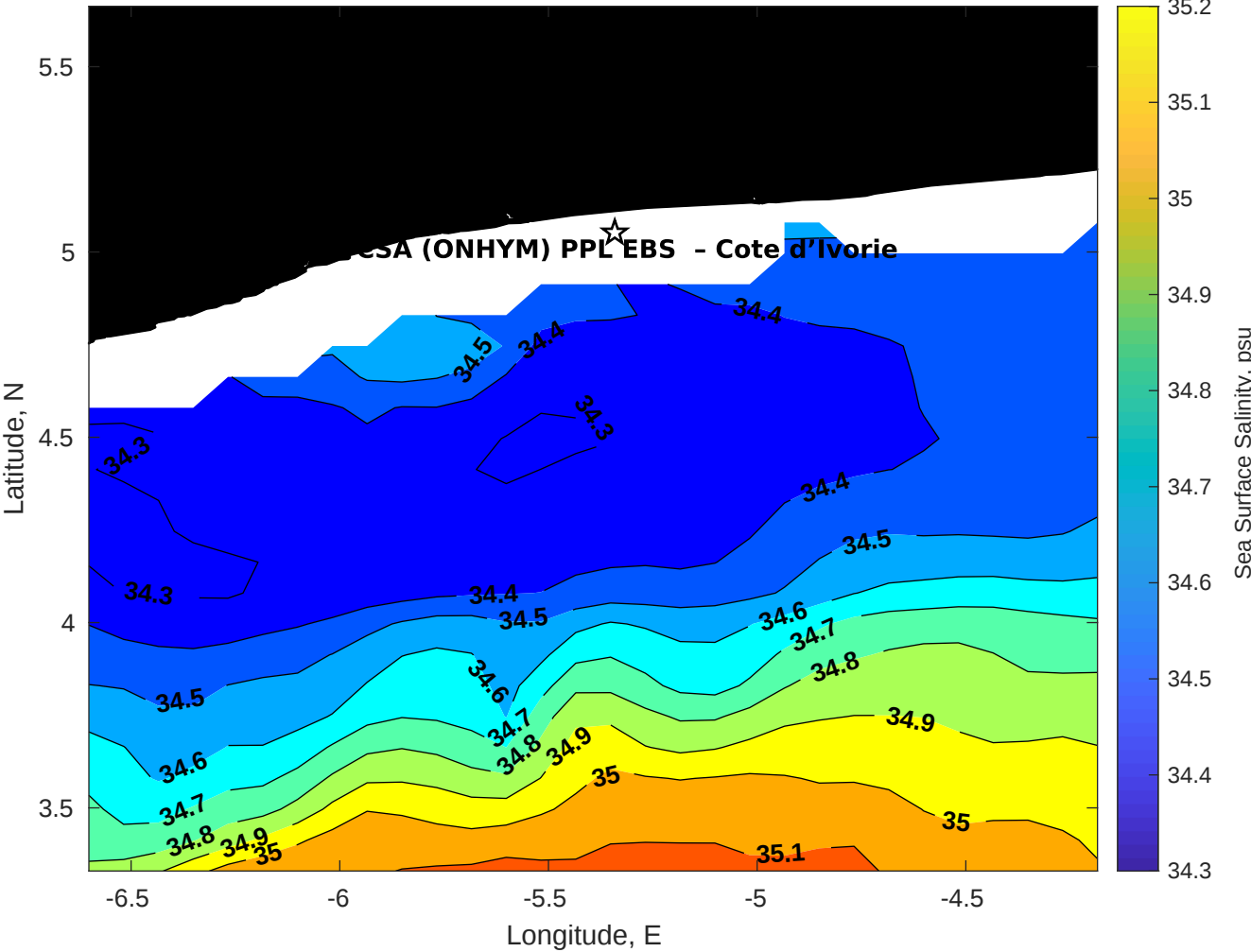
Surface Salinity for CSA (ONHYM) PPL EBS - Cote d'Ivoire at 24-Nov-2025 00:00:00
