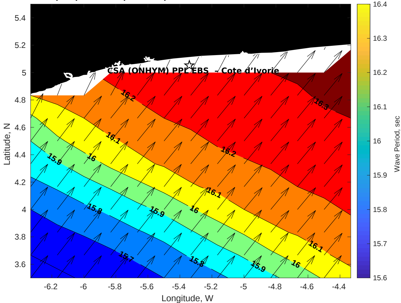
GFS Wave Period (sec) for CSA (ONHYM) PPL EBS - Cote d'Ivoire at 25-Nov-2025 09:00:00
